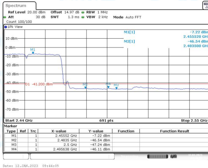
11N40SISO_Ant1_High_2452_Peak
