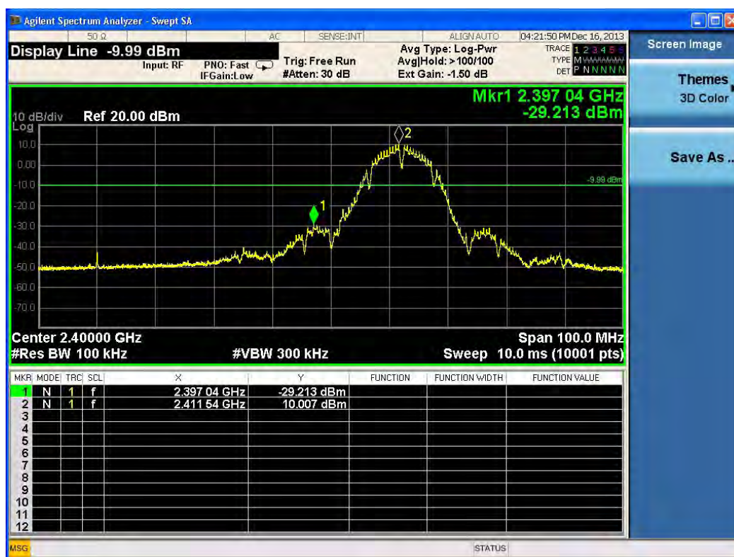
Channel 1 (2412MHz)
