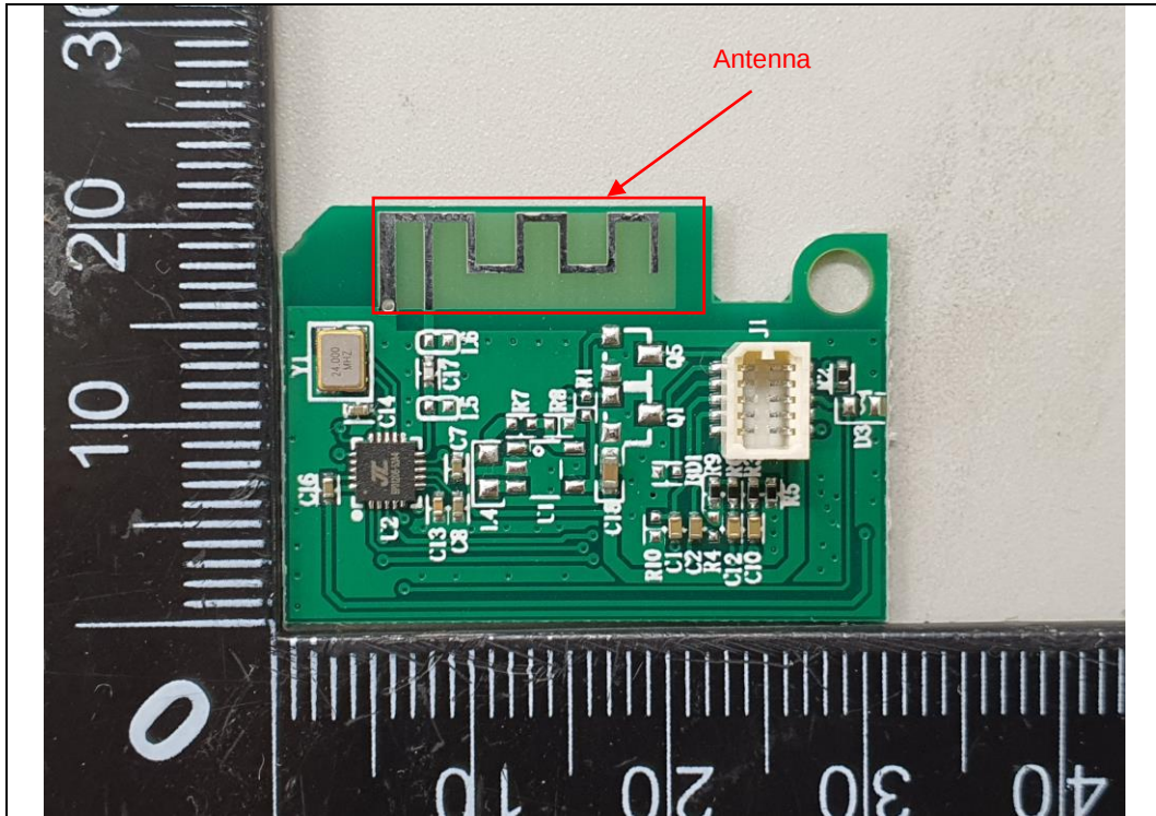
RF Board Front
