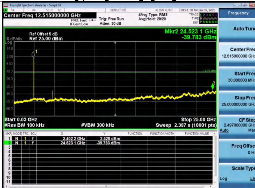
2 Spurious Emissions BT 1-DH5 2402
