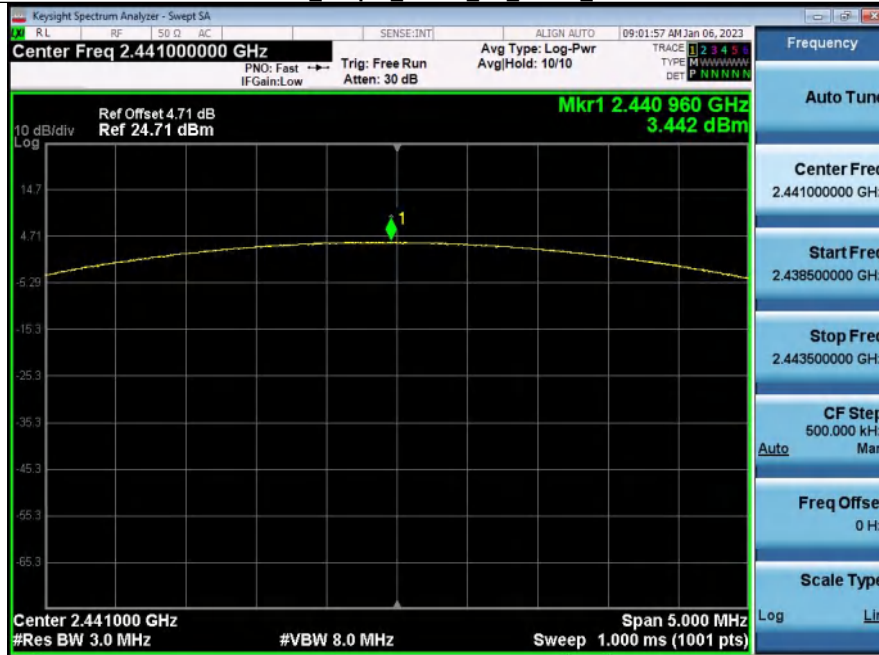
Peak Output Power_BT_3-DH5_2441
