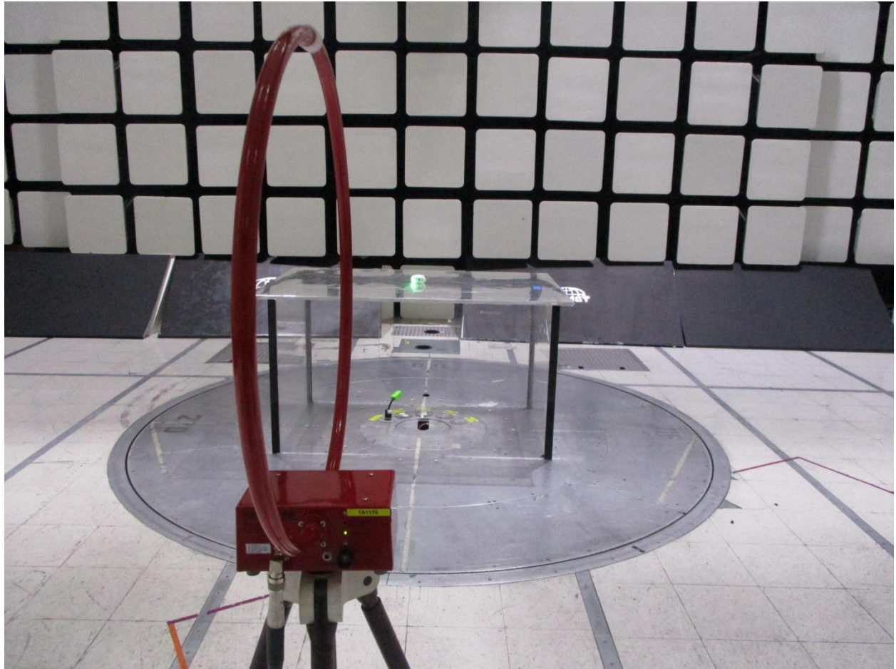
Radiated Emissions 9kHz – 30MHz
