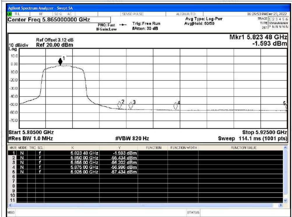
Restrict Band NVNT n20 5825MHz Ant1 Average
