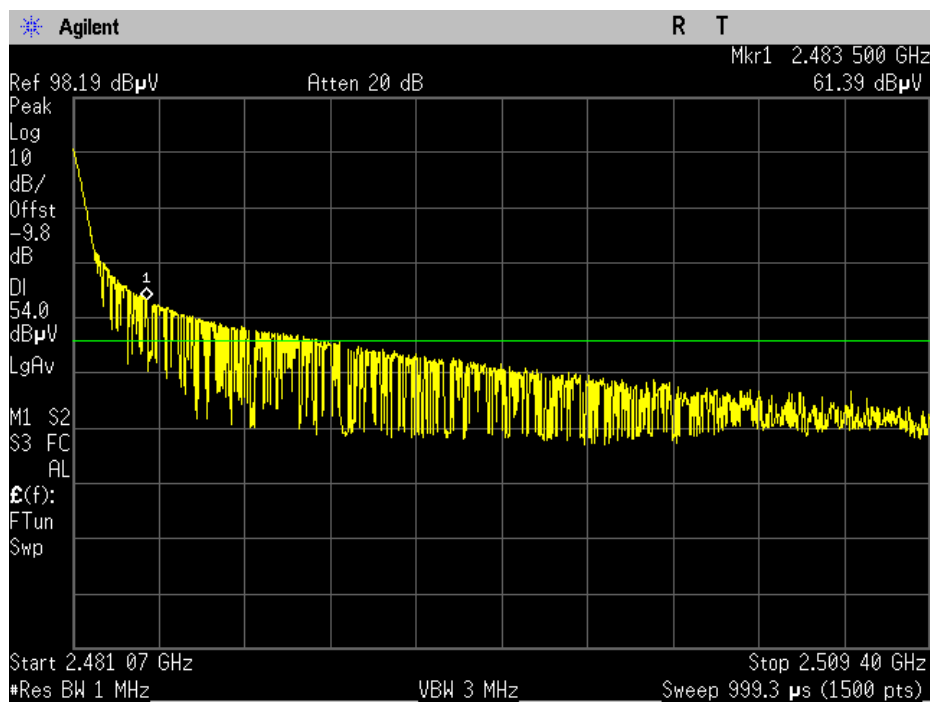
High channel restricted band edge - Peak
