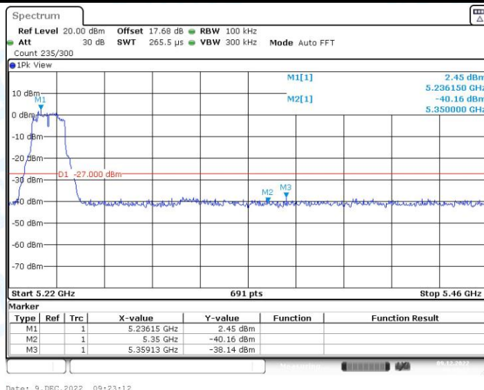
11A-CDD_Ant2_High_5240
