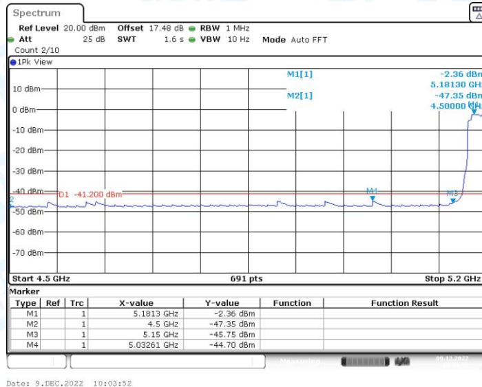
11N40MIMO_Ant1_Low_5190_Peak
