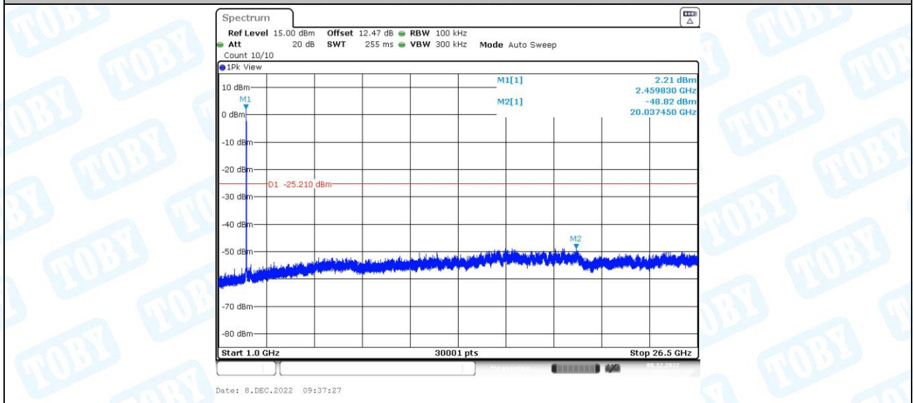
11G-CDD_Ant2_2462_0~Reference
