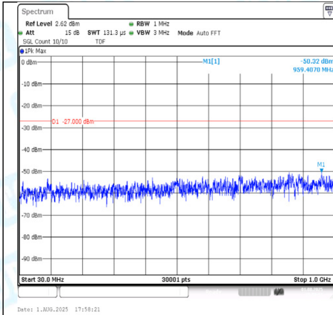
11A-CDD-Ant1-5200-30~1000-PASS
