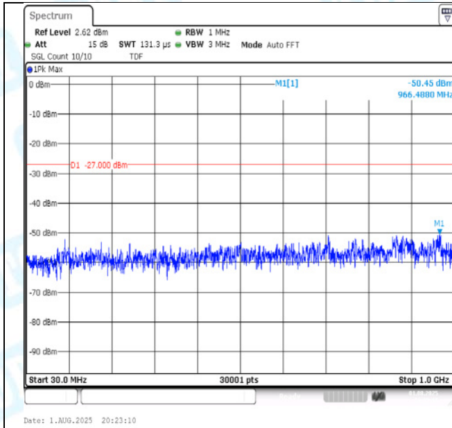
11N40-CDD-Ant1-5190-30~1000-PASS
