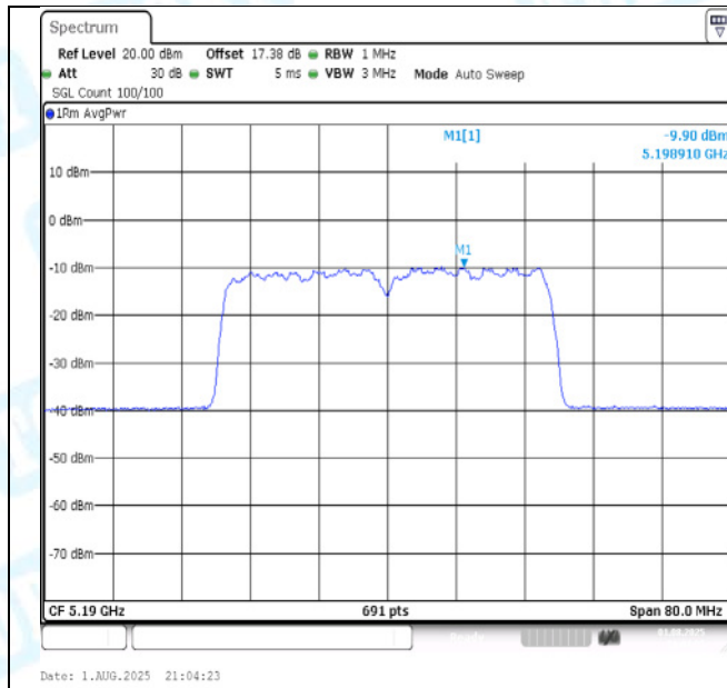
11AX40MIMO-Ant1-5190-PASS
