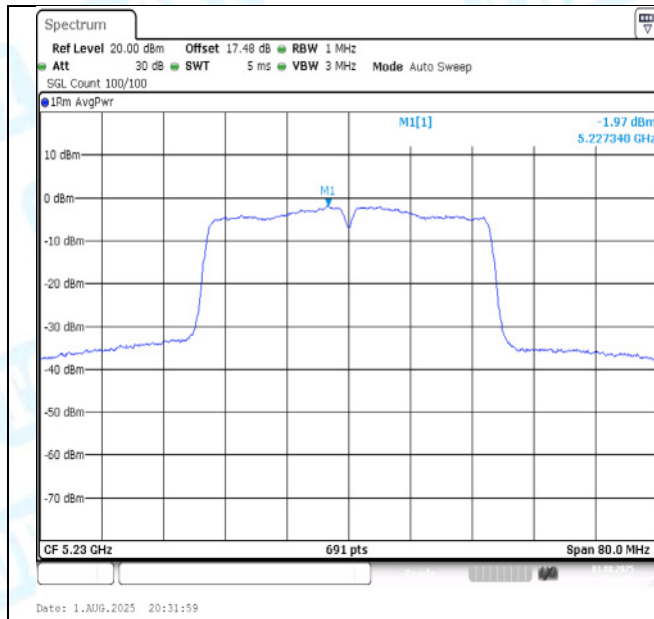
11N40-CDD-Ant1-5230-PASS
