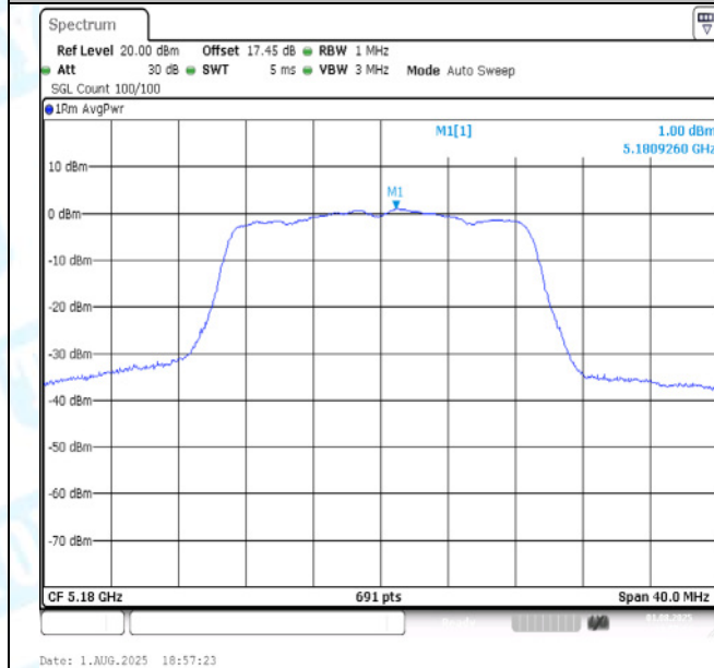
11N20-CDD-Ant1-5180-PASS
