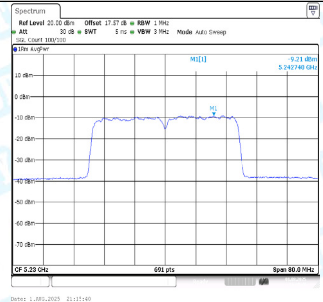
11AX40MIMO-Ant2-5230-PASS
