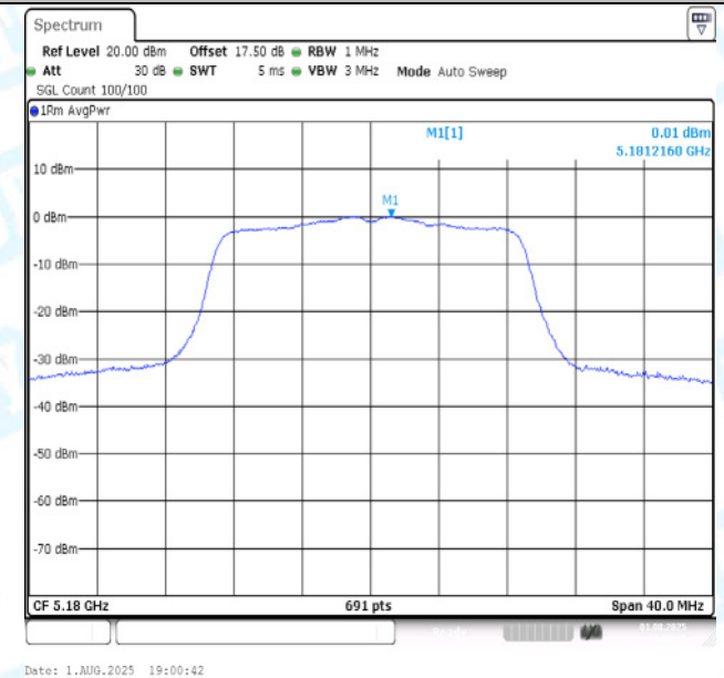
11N20-CDD-Ant2-5180-PASS
