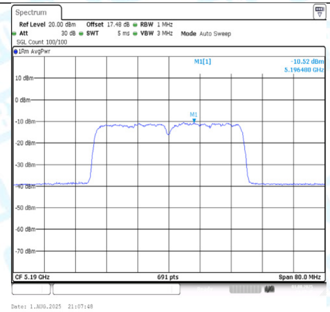
11AX40MIMO-Ant2-5190-PASS
