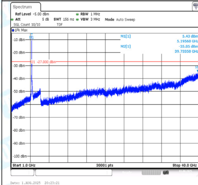
11N40-CDD-Ant1-5190-1000~40000-PASS
