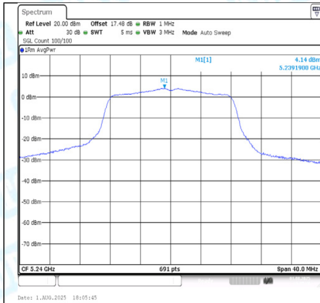
11A-CDD-Ant1-5240-PASS
