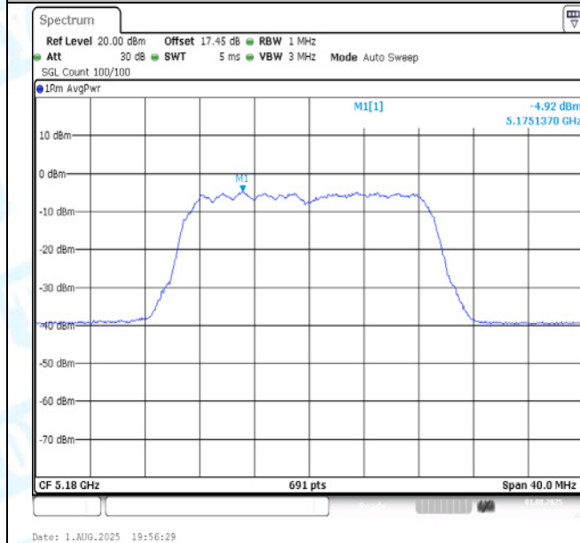
11AC20MIMO-Ant1-5180-PASS
