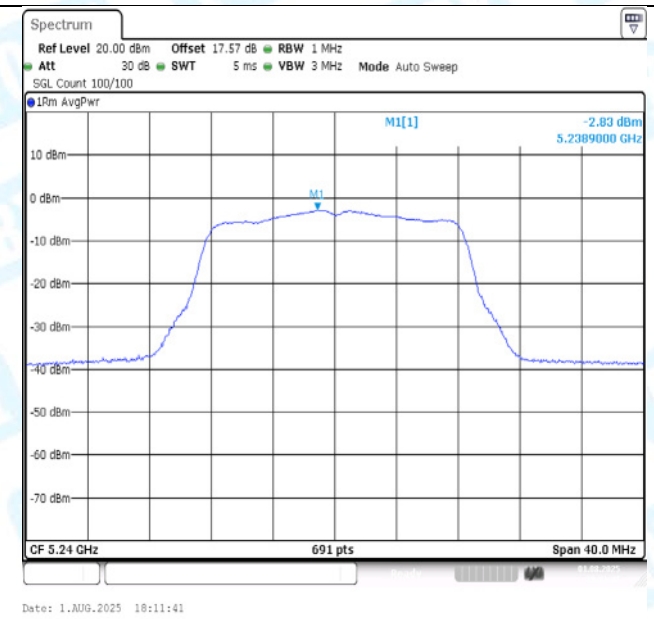
11A-CDD-Ant2-5240-PASS
