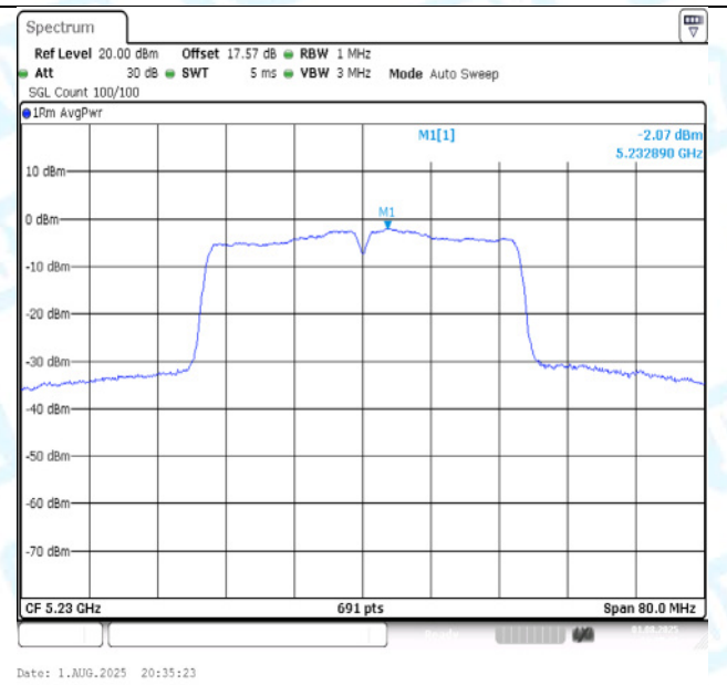
11N40-CDD-Ant2-5230-PASS
