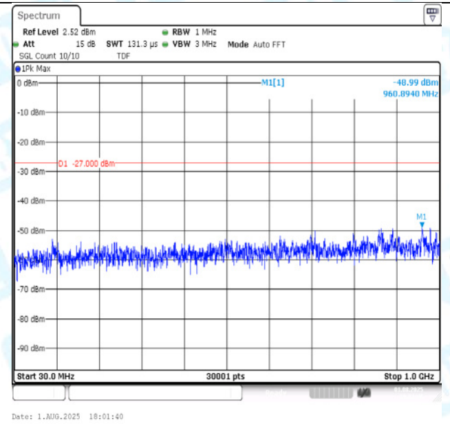
11A-CDD-Ant2-5200-30~1000-PASS
