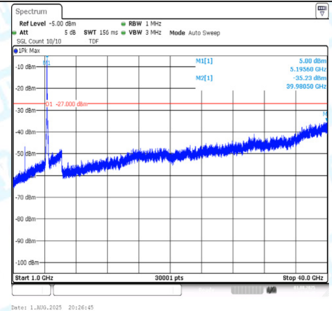
11N40-CDD-Ant2-5190-1000~40000-PASS
