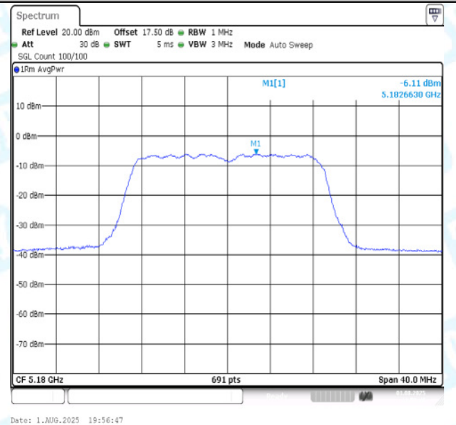
11AC20MIMO-Ant2-5180-PASS
