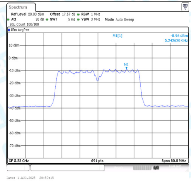
11AC40MIMO-Ant2-5230-PASS
