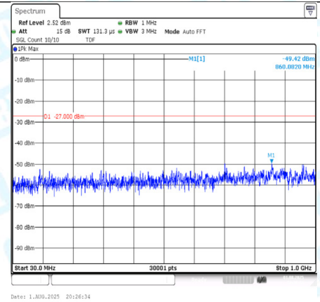
11N40-CDD-Ant2-5190-30~1000-PASS
