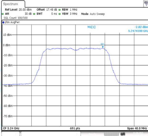
11AC20MIMO-Ant1-5200-PASS
