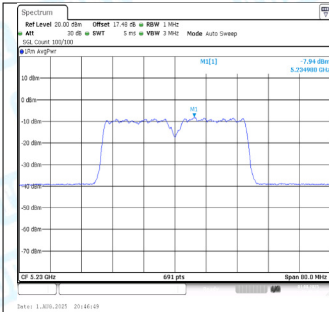
11AC40MIMO-Ant1-5230-PASS
