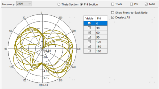
Phi Section
