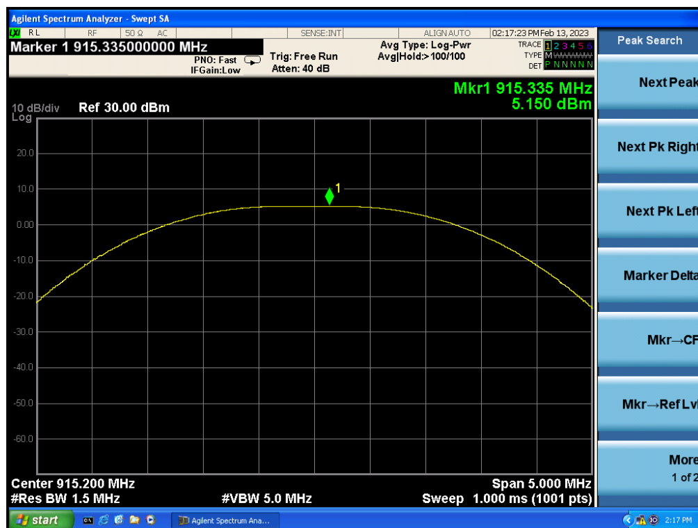
Peak output Power plot on channel 01
