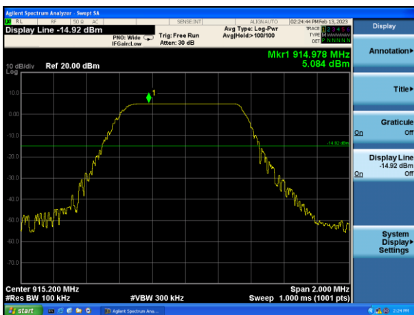
LoRa on channel 01
