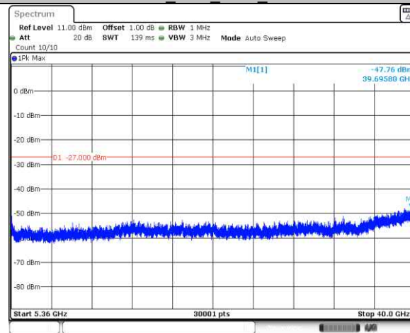
11AC20SISO Ant1 5320 5360~40000
