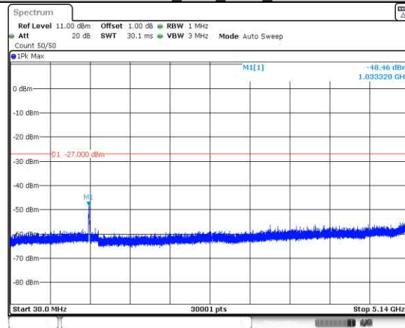
11N20SISO Ant1 5240 30-5140
