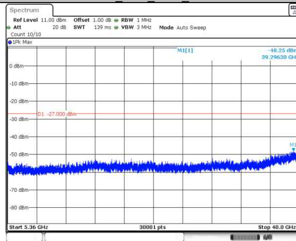
11N20SISO Ant1 5200 5360-40000
