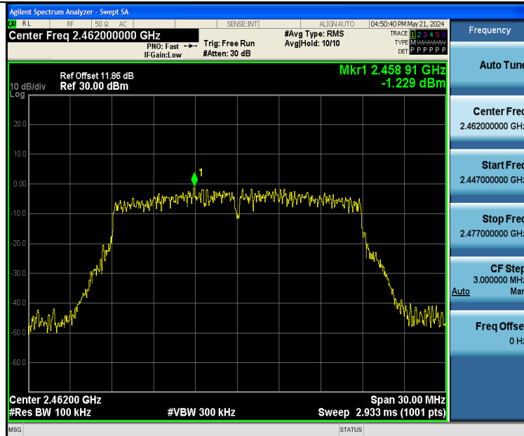
11N20SISO-Ant1-2462-0~Reference-PASS
