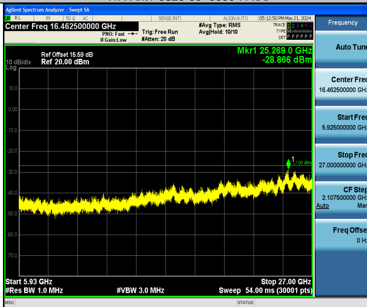
11A-Ant1-5825-5925~27000-PASS
