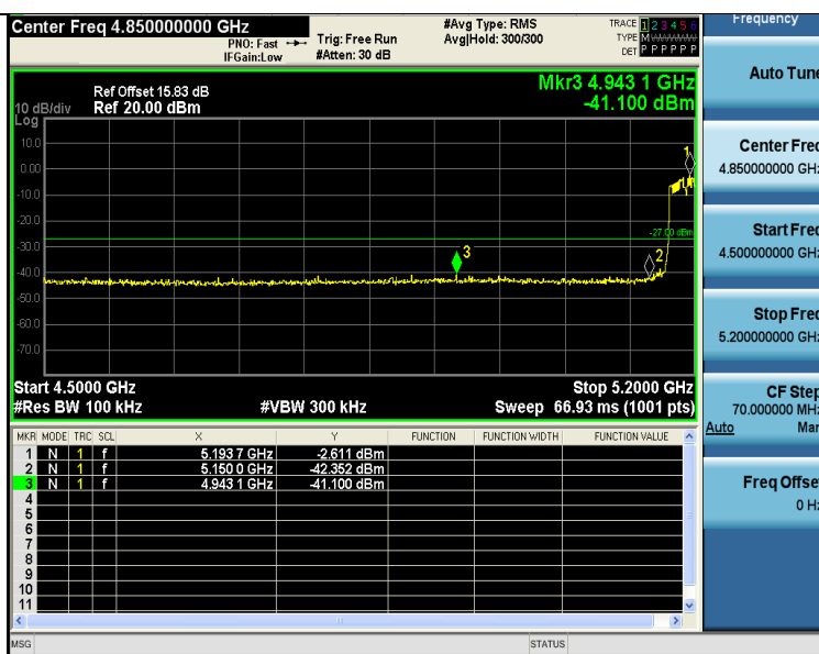
11N40SISO-Ant1-5190-PASS
