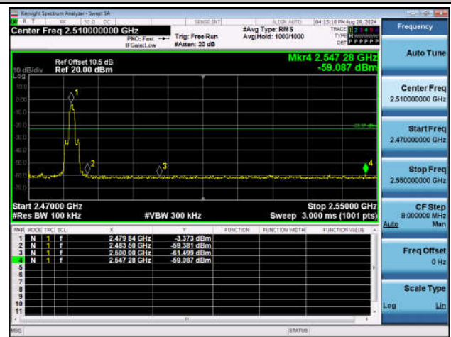
3DH5-Ant1-Hop_2480-PASS
