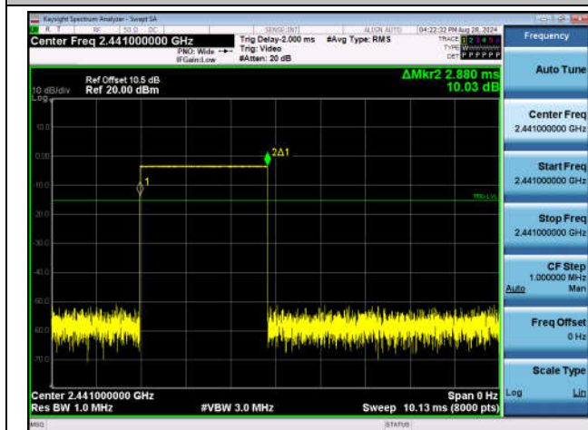
2DH5-Ant1-Hop-PASS
