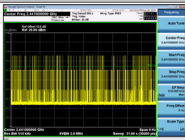
3DH5-Ant1-Hop-PASS
