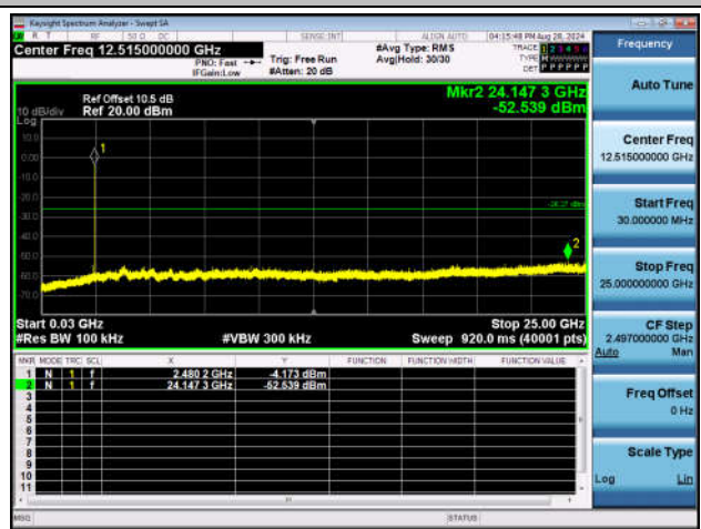
3DH5-Ant1-2480-30~25000-PASS
