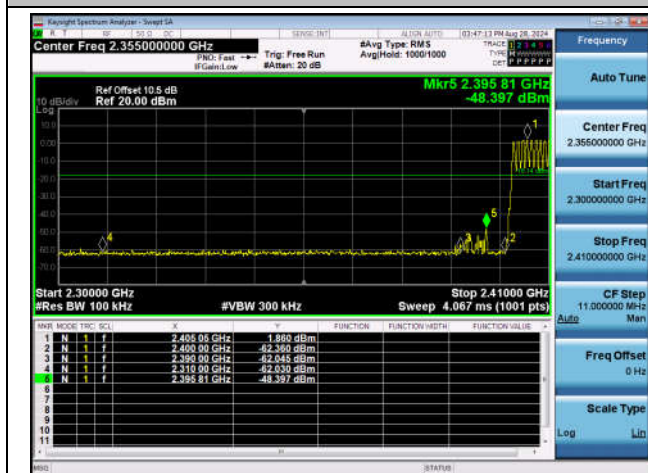
2DH5-Ant1-2402-PASS
