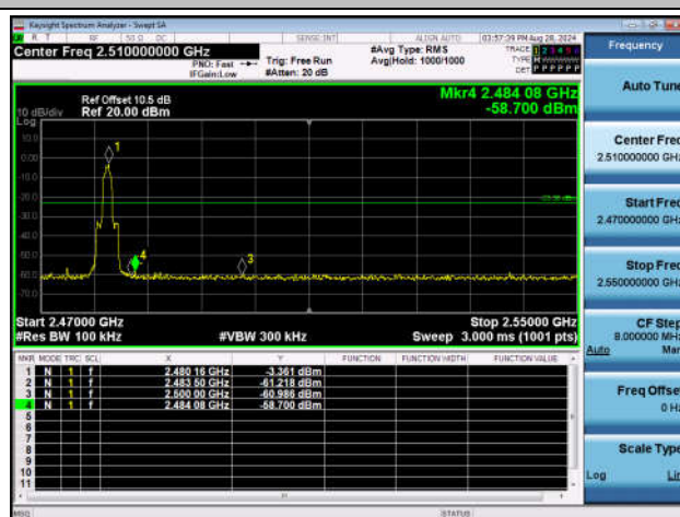
2DH5-Ant1-2480-PASS
