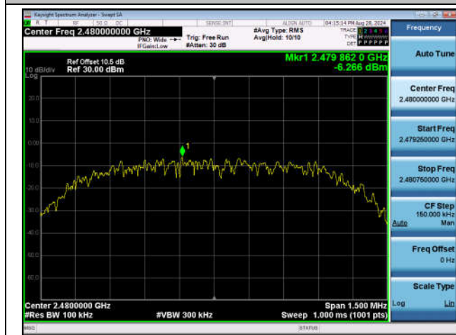
3DH5-Ant1-2480-0~Reference-PASS
