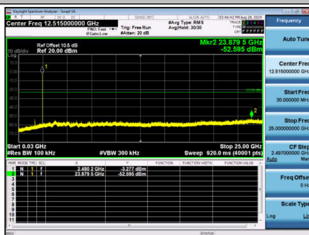
DH5-Ant1-2480-30~25000-PASS
