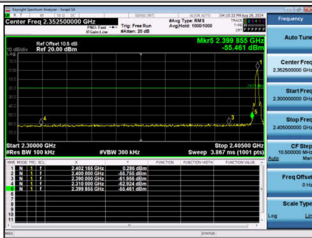
3DH5-Ant1-Hop_2402-PASS
