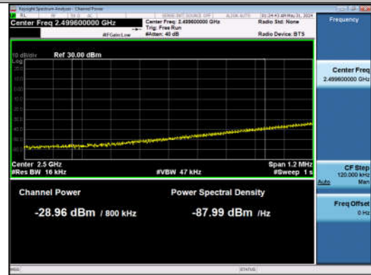
20MHz-20MHz_QPSK@QPSK-QPSK@QPSK_20850-21048_1RB#0@100RB#0-0RB#0@100RB#0_Final1
