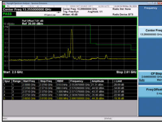
20MHz-15MHz_QPSK@QPSK-QPSK@QPSK_21201-2137 2_1RB#99@100RB#0-0RB#0@75RB#0
