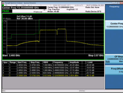
20MHz-10MHz_QPSK@QPSK-QPSK@QPSK_20850-20994_100RB#0@100RB#0-50RB#0@50RB#0
