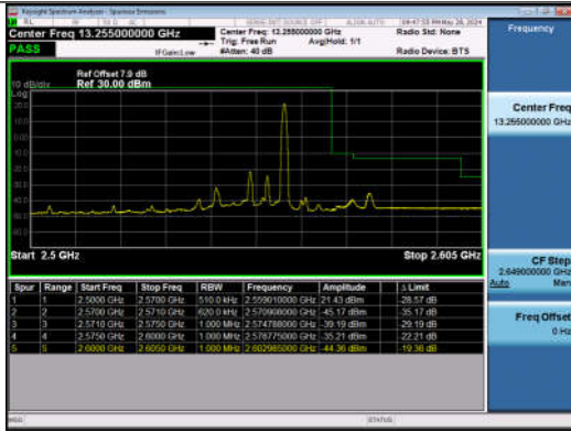
20MHz-10MHz_QPSK@QPSK-QPSK@QPSK_21251-2139 5_1RB#99@100RB#0-0RB#0@50RB#0
