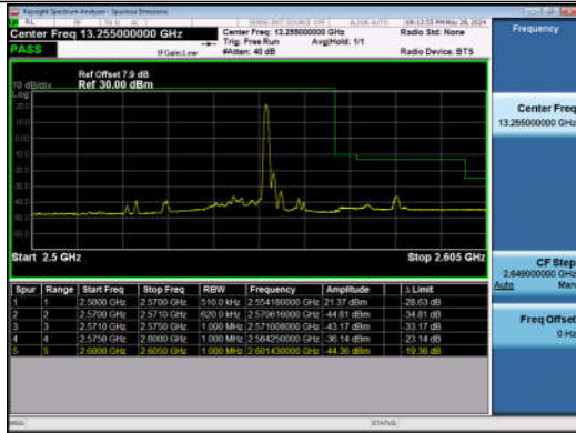
15MHz-15MHz_QPSK@QPSK-QPSK@QPSK_21225-2137 5_1RB#74@75RB#0-0RB#0@75RB#0
