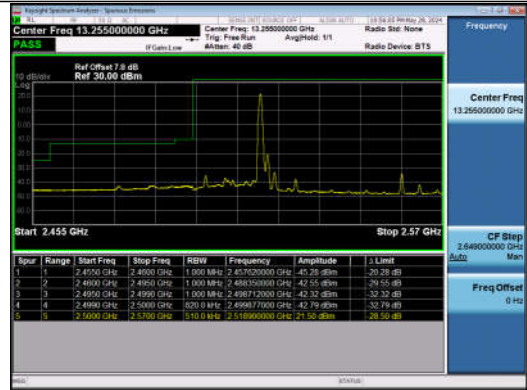
20MHz-20MHz_QPSK@QPSK-QPSK@QPSK_20850-210 48_1RB#99@100RB#0-0RB#0@100RB#0
