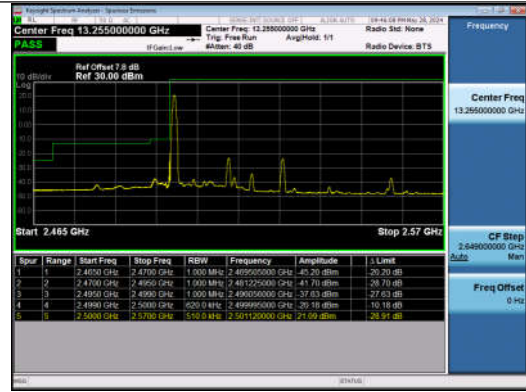
20MHz-10MHz_QPSK@QPSK-QPSK@QPSK_20850-20994_1RB#0@100RB#0-0RB#0@50RB#0
