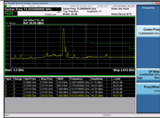
20MHz-20MHz_QPSK@QPSK-QPSK@QPSK_21152-21350_1RB#99@100RB#0-0RB#0@100RB#0
