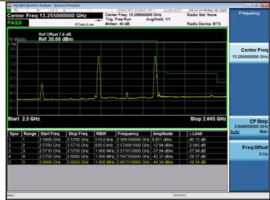
15MHz-15MHz_QPSK@QPSK-QPSK@QPSK_21225-2137 75_1RB#0@75RB#0-1RB#74@75RB#0
