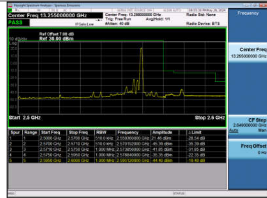
15MHz-10MHz_QPSK@QPSK-QPSK@QPSK_21277-21397_1RB#74@75RB#0-0RB#0@50RB#0
