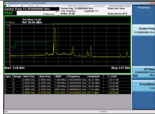
20MHz-15MHz_QPSK@QPSK-QPSK@QPSK_20850-210 21_1RB#0@100RB#0-0RB#0@75RB#0
