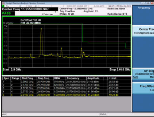
20MHz-20MHz_QPSK@QPSK-QPSK@QPSK_21152-21350_350_1RB#0@100RB#0-0RB#0@100RB#0
