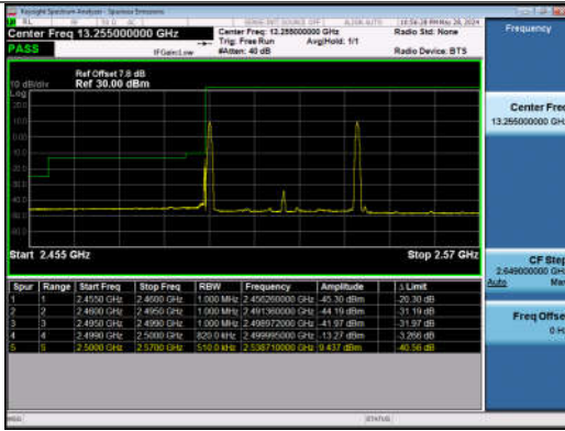
20MHz-20MHz_QPSK@QPSK-QPSK@QPSK_20850-21048_1RB#0@100RB#0-1RB#99@100RB#0
