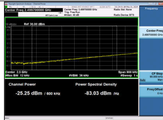
15MHz-15MHz_QPSK@QPSK-QPSK@QPSK_20825-20975_1RB#0@75RB#0-0RB#0@75RB#0_Final1
