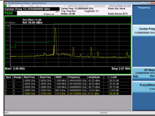
15MHz-20MHz_QPSK@QPSK-QPSK@QPSK_20828-209 99_1RB#0@75RB#0-0RB#0@100RB#0
