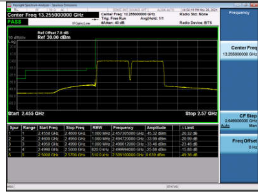
20MHz-20MHz_QPSK@QPSK-QPSK@QPSK_20850-21048_100RB#0@100RB#0-100RB#0@100RB#0
