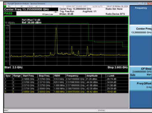
20MHz-10MHz_QPSK@QPSK-QPSK@QPSK_21251-21395_1RB#0@100RB#0-0RB#0@50RB#0
