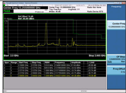
15MHz-15MHz_QPSK@QPSK-QPSK@QPSK_21225-2137 75_1RB#0@75RB#0-0RB#0@75RB#0
