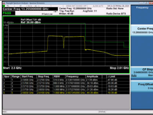
15MHz-20MHz_QPSK@QPSK-QPSK@QPSK_21179-2135_0_75RB#0@75RB#0-100RB#0@100RB#0
