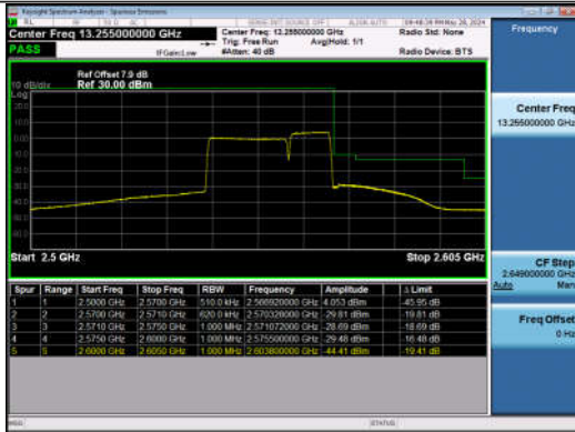
20MHz-10MHz_QPSK@QPSK-QPSK@QPSK_21251-2139 5_100RB#0@100RB#0-50RB#0@50RB#0
