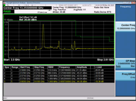
20MHz-15MHz_QPSK@QPSK-QPSK@QPSK_21201-213 72_1RB#0@100RB#0-0RB#0@75RB#0
