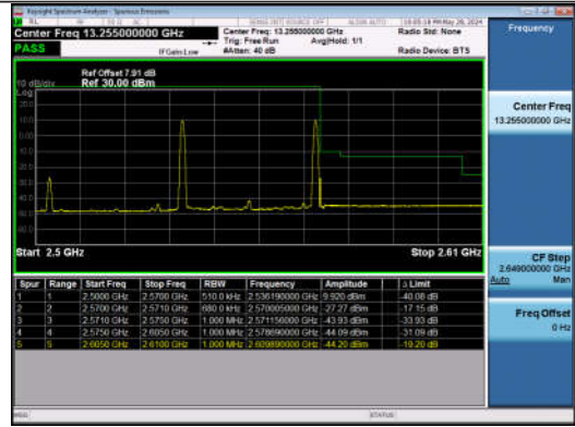
20MHz-15MHz_QPSK@QPSK-QPSK@QPSK_21201-213 72_1RB#0@100RB#0-1RB#74@75RB#0
