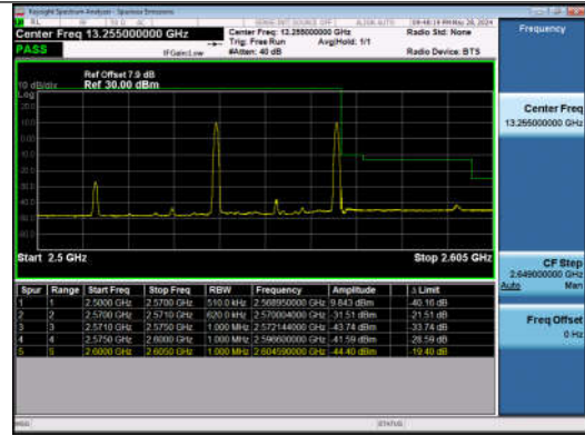
20MHz-10MHz_QPSK@QPSK-QPSK@QPSK_21251-213 95_1RB#0@100RB#0-1RB#49@50RB#0
