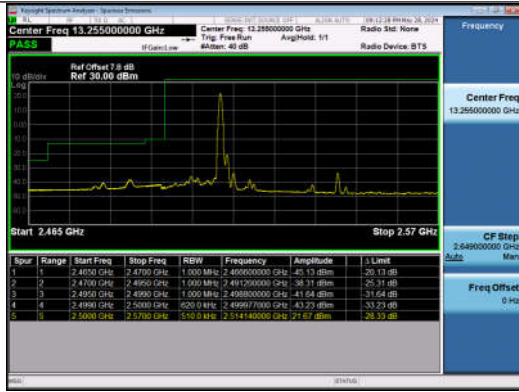
15MHz-15MHz_QPSK@QPSK-QPSK@QPSK_20825-2097 5_1RB#74@75RB#0-0RB#0@75RB#0
