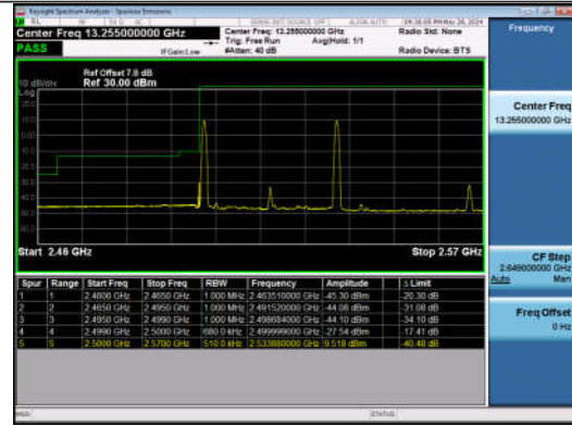
15MHz-20MHz_QPSK@QPSK-QPSK@QPSK_20828-209 99_1RB#0@75RB#0-1RB#99@100RB#0
