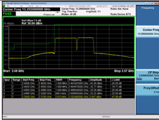
20MHz-15MHz_QPSK@QPSK-QPSK@QPSK_20850-2102 1_100RB#0@100RB#0-75RB#0@75RB#0
