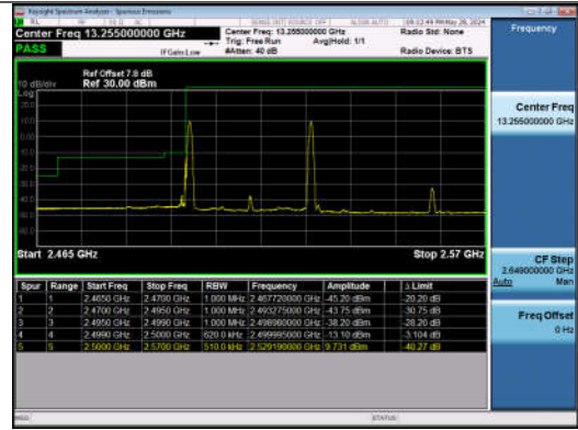
15MHz-15MHz_QPSK@QPSK-QPSK@QPSK_20825-2097 75_1RB#0@75RB#0-1RB#74@75RB#0
