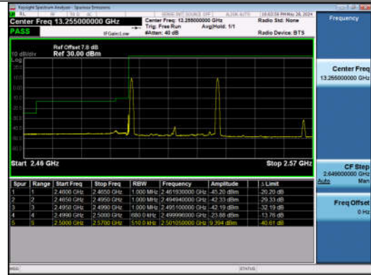
20MHz-15MHz_QPSK@QPSK-QPSK@QPSK_20850-210 21_1RB#0@100RB#0-1RB#74@75RB#0
