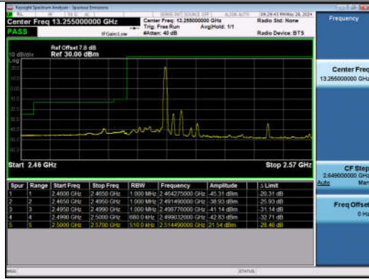
15MHz-20MHz_QPSK@QPSK-QPSK@QPSK_20828-209 99_1RB#74@75RB#0-0RB#0@100RB#0
