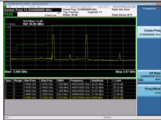
20MHz-10MHz_QPSK@QPSK-QPSK@QPSK_20850-20994_1RB#0@100RB#0-1RB#49@50RB#0
