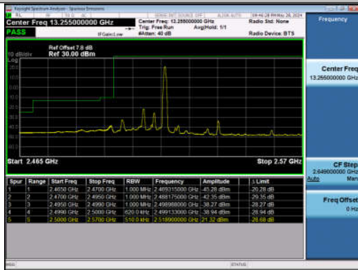
20MHz-10MHz_QPSK@QPSK-QPSK@QPSK_20850-20994_1RB#99@100RB#0-0RB#0@50RB#0
