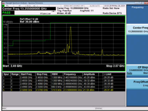
20MHz-15MHz_QPSK@QPSK-QPSK@QPSK_20850-2102 1_1RB#99@100RB#0-0RB#0@75RB#0
