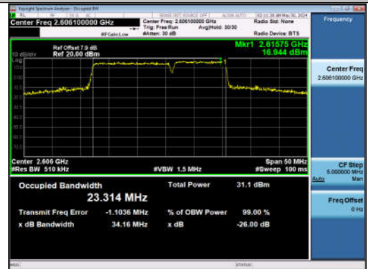
41-41-15MHz-10MHz-16QAM-16QAM-40691-40811-75RB#0-50RB#0-PASS
