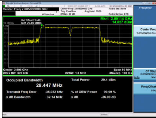
41-41-15MHz-15MHz-QPSK-QPSK-40665-40815-75RB#0 -75RB#0-PASS
