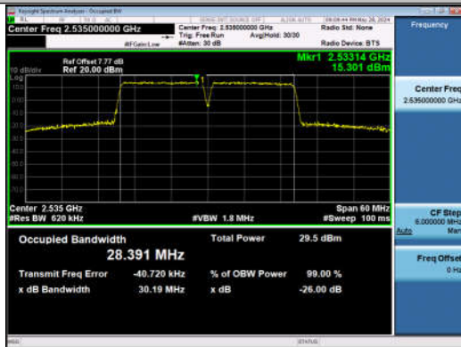
7-7-15MHz-15MHz-QPSK-QPSK-21025-21175-75RB#0-7 5RB#0-PASS
