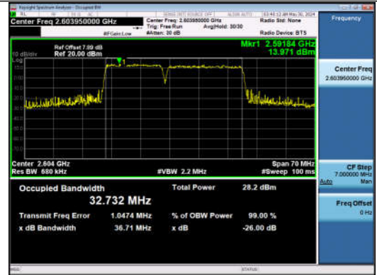
41-41-15MHz-20MHz-16QAM-16QAM-40644-40815-75RB# 0-100RB#0-PASS
