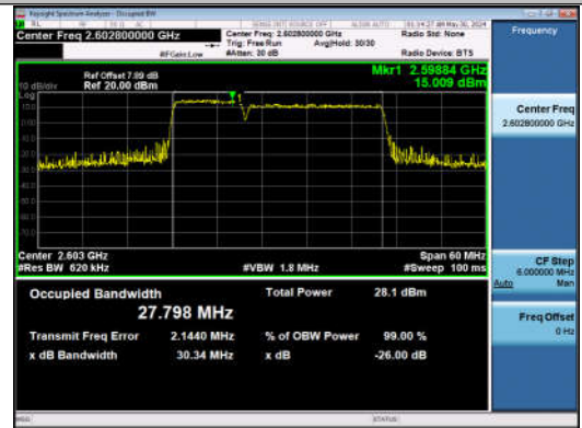
41-41-10MHz-20MHz-16QAM-16QAM-40646-40790-50RB#0-100RB#0-PASS
