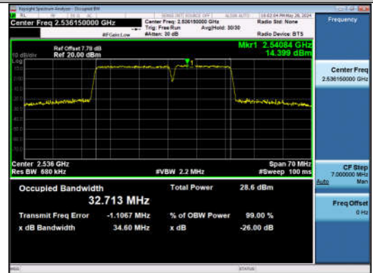
7-7-20MHz-15MHz-16QAM-16QAM-21026-21197-100RB#0- 75RB#0-PASS
