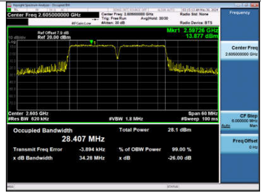
41-41-15MHz-15MHz-16QAM-16QAM-40665-40815-75RB# 0-75RB#0-PASS
