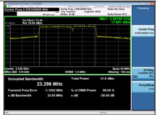
7-7-15MHz-10MHz-16QAM-16QAM-21051-21171-75RB#0-5 0RB#0-PASS
