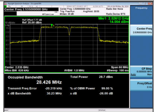
7-7-15MHz-15MHz-16QAM-16QAM-21025-21175-75RB#0-7 5RB#0-PASS
