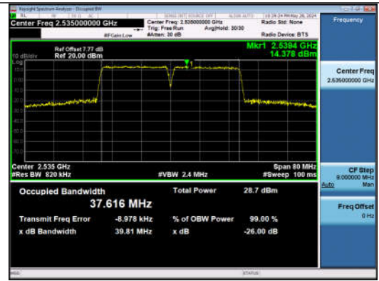
7-7-20MHz-20MHz-16QAM-16QAM-21001-21199-100RB#0-100RB#0-PASS
