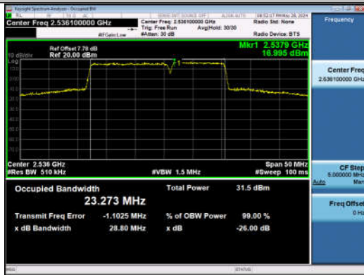
7-7-15MHz-10MHz-QPSK-QPSK-21051-21171-75RB#0-5 0RB#0-PASS
