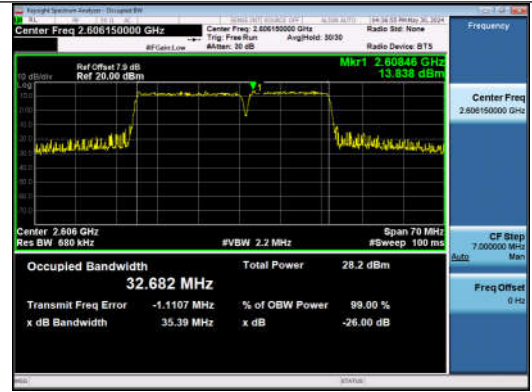
41-41-20MHz-15MHz-16QAM-16QAM-40666-40837-100RB #0-75RB#0-PASS
