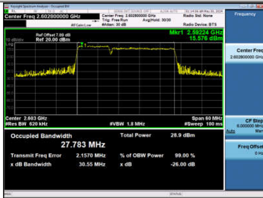
41-41-10MHz-20MHz-QPSK-QPSK-40646-40790-50RB#0-100RB#0-PASS
