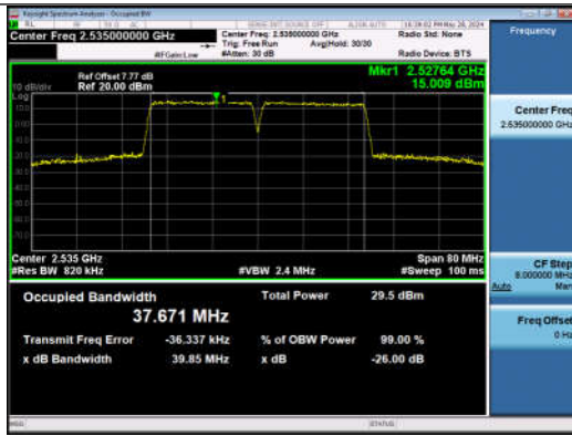
7-7-20MHz-20MHz-QPSK-QPSK-21001-21199-100RB#0-100RB#0-PASS
