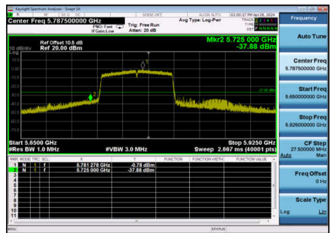
U-NII-3 ,Plot 1,Band Edge-802.11ac(80 MHz),5775MHz,Ant1
