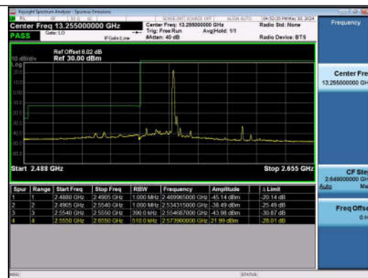
20MHz-20MHz_QPSK@QPSK-QPSK@QPSK_40340-40538 _1RB#99@100RB#0-0RB#0@100RB#0
