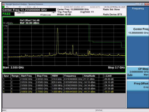
20MHz-20MHz_QPSK@QPSK-QPSK@QPSK_40942-41 140_1RB#0@100RB#0-0RB#0@100RB#0
