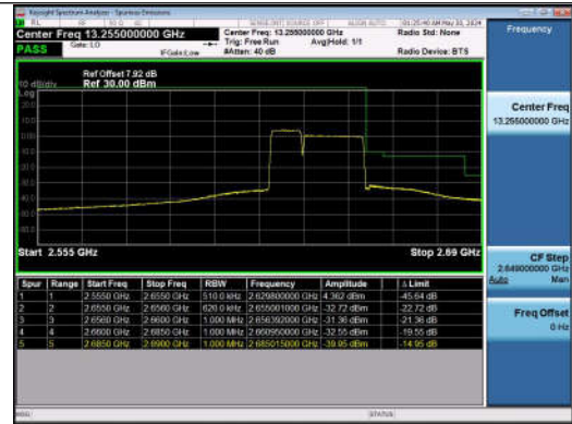
10MHz-20MHz_QPSK@QPSK-QPSK@QPSK_40996-41140 _50RB#0@50RB#0-100RB#0@100RB#0
