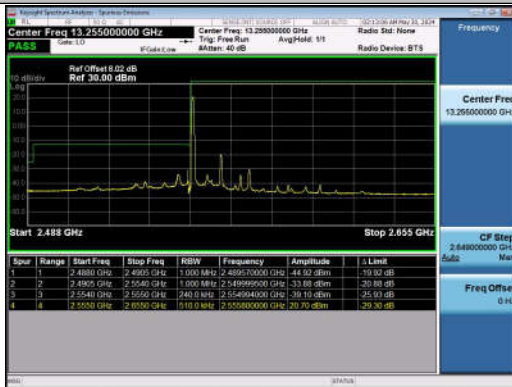
15MHz-10MHz_QPSK@QPSK-QPSK@QPSK_40315-40 435_1RB#0@75RB#0-0RB#0@50RB#0
