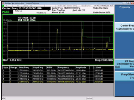
20MHz-15MHz_QPSK@QPSK-QPSK@QPSK_40991-41 162_1RB#0@100RB#0-1RB#74@75RB#0
