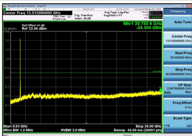
FDD04_MidRange_20MHz_30MHz~26GHz
