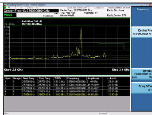
15MHz-10MHz_QPSK@QPSK-QPSK@QPSK_21277-21397_1RB#74@75RB#0-0RB#0@50RB#0
