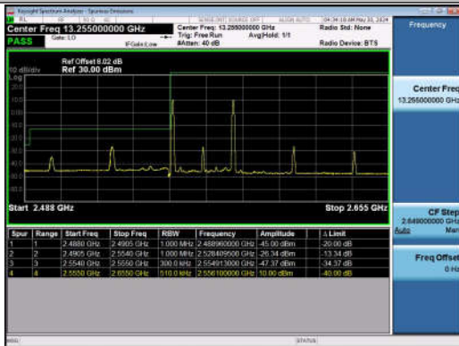
20MHz-10MHz_QPSK@QPSK-QPSK@QPSK_40340-40484_1RB#0@100RB#0-1RB#49@50RB#0
