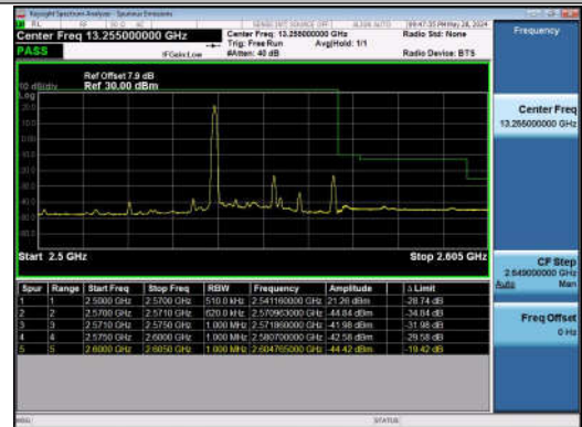
20MHz-10MHz_QPSK@QPSK-QPSK@QPSK_21251-21395_1RB#0@100RB#0-0RB#0@50RB#0
