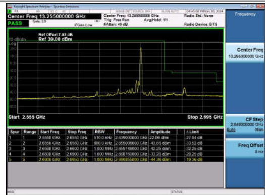
20MHz-15MHz_QPSK@QPSK-QPSK@QPSK_40991-41162 _1RB#99@100RB#0-0RB#0@75RB#0
