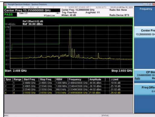
15MHz-20MHz_QPSK@QPSK-QPSK@QPSK_40318-40489 _1RB#74@75RB#0-0RB#0@100RB#0
