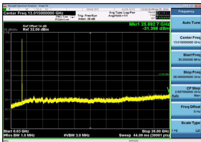
FDD04_HighRange_20MHz_30MHz~26GHz
