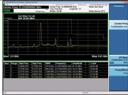
20MHz-15MHz_QPSK@QPSK-QPSK@QPSK_21201-213_72_1RB#0@100RB#0-0RB#0@75RB#0
