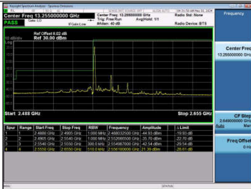
20MHz-10MHz_QPSK@QPSK-QPSK@QPSK_40340-40484_1RB#0@100RB#0-0RB#0@50RB#0
