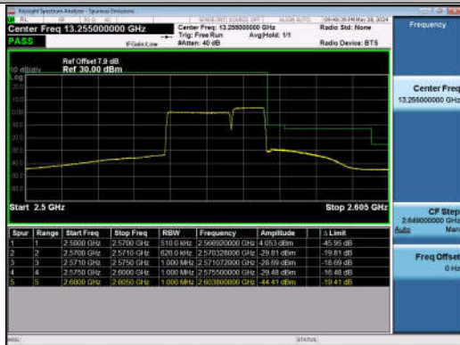
20MHz-10MHz_QPSK@QPSK-QPSK@QPSK_21251-2139 5_100RB#0@100RB#0-50RB#0@50RB#0
