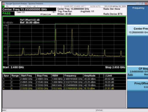
15MHz-10MHz_QPSK@QPSK-QPSK@QPSK_40315-40 435_1RB#0@75RB#0-1RB#49@50RB#0
