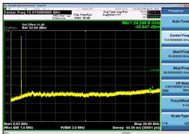
FDD26_Part 22_HighRange_15MHz_30MHz~26GHz
