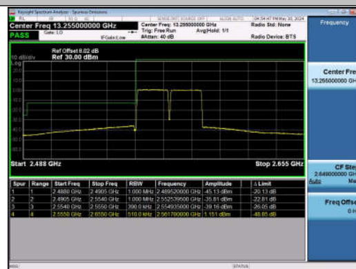
20MHz-20MHz_QPSK@QPSK-QPSK@QPSK_40340-40538 _100RB#0@100RB#0-100RB#0@100RB#0
