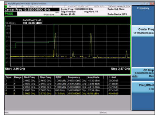
15MHz-20MHz_QPSK@QPSK-QPSK@QPSK_20828-209 99_1RB#0@75RB#0-1RB#99@100RB#0
