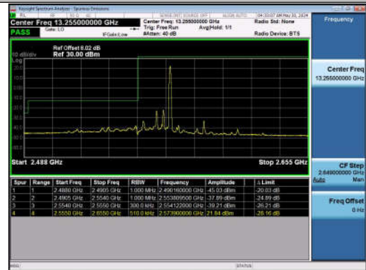
20MHz-10MHz_QPSK@QPSK-QPSK@QPSK_40340-40484_1RB#99@100RB#0-0RB#0@50RB#0
