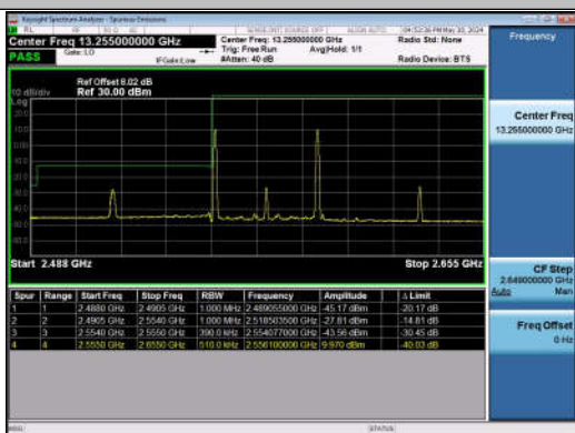
20MHz-20MHz_QPSK@QPSK-QPSK@QPSK_40340-40 538_1RB#0@100RB#0-1RB#99@100RB#0
