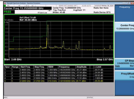
20MHz-15MHz_QPSK@QPSK-QPSK@QPSK_20850-210 21_1RB#0@100RB#0-0RB#0@75RB#0
