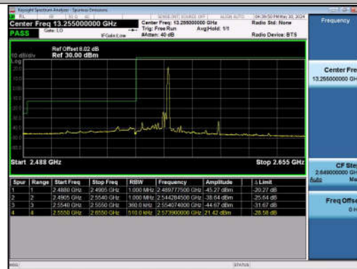
20MHz-15MHz_QPSK@QPSK-QPSK@QPSK_40340-40511 _1RB#99@100RB#0-0RB#0@75RB#0
