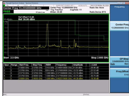
15MHz-15MHz_QPSK@QPSK-QPSK@QPSK_21225-213 75_1RB#0@75RB#0-0RB#0@75RB#0
