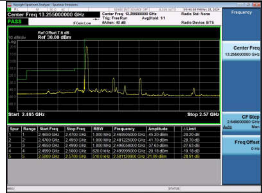
20MHz-10MHz_QPSK@QPSK-QPSK@QPSK_20850-20994_1RB#0@100RB#0-0RB#0@50RB#0
