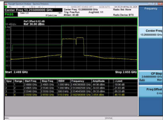
20MHz-10MHz_QPSK@QPSK-QPSK@QPSK_40340-40484_100RB#0@100RB#0-50RB#0@50RB#0
