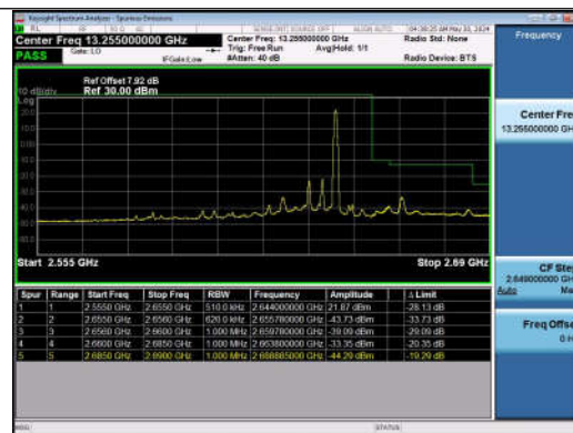
20MHz-10MHz_QPSK@QPSK-QPSK@QPSK_41041-41185 _1RB#99@100RB#0-0RB#0@50RB#0
