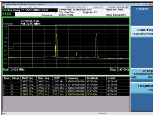
20MHz-20MHz_QPSK@QPSK-QPSK@QPSK_20850-21048_1RB#0@100RB#0-1RB#99@100RB#0
