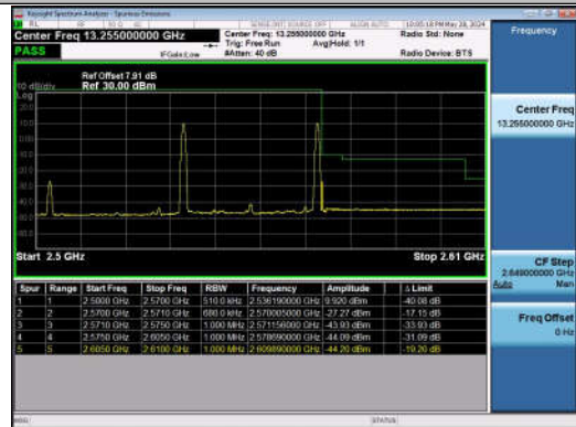
20MHz-15MHz_QPSK@QPSK-QPSK@QPSK_21201-213_72_1RB#0@100RB#0-1RB#74@75RB#0
