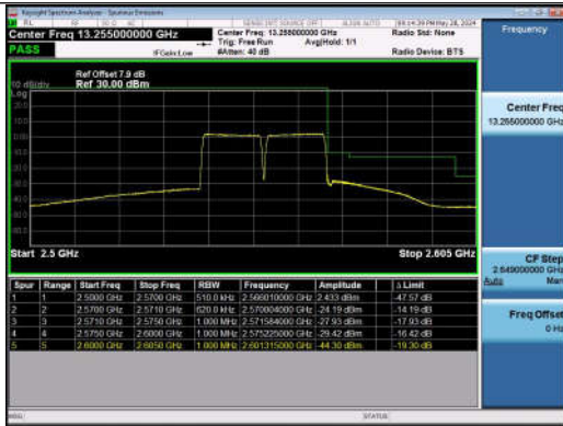
15MHz-15MHz_QPSK@QPSK-QPSK@QPSK_21225-213 75_75RB#0@75RB#0-75RB#0@75RB#0
