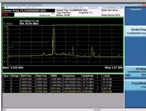
20MHz-20MHz_QPSK@QPSK-QPSK@QPSK_20850-21048_1RB#0@100RB#0-0RB#0@100RB#0
