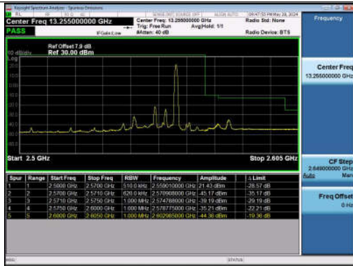
20MHz-10MHz_QPSK@QPSK-QPSK@QPSK_21251-2139 5_1RB#99@100RB#0-0RB#0@50RB#0
