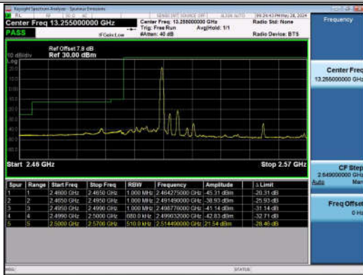
15MHz-20MHz_QPSK@QPSK-QPSK@QPSK_20828-209 99_1RB#74@75RB#0-0RB#0@100RB#0
