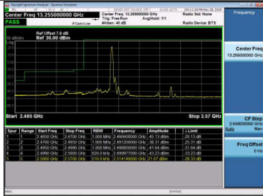
15MHz-15MHz_QPSK@QPSK-QPSK@QPSK_20825-2097 5_1RB#74@75RB#0-0RB#0@75RB#0
