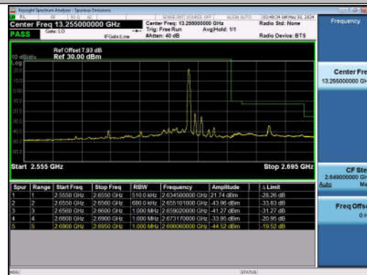
15MHz-20MHz_QPSK@QPSK-QPSK@QPSK_40969-41140 _1RB#74@75RB#0-0RB#0@100RB#0
