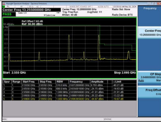
15MHz-20MHz_QPSK@QPSK-QPSK@QPSK_40969-41140_1RB#0@75RB#0-1RB#99@100RB#0
