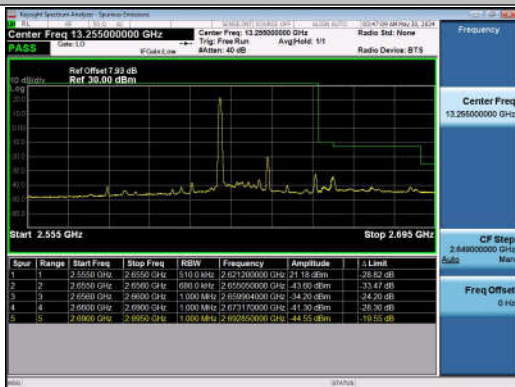
15MHz-20MHz_QPSK@QPSK-QPSK@QPSK_40969-41 140_1RB#0@75RB#0-0RB#0@100RB#0
