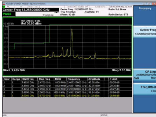
20MHz-10MHz_QPSK@QPSK-QPSK@QPSK_20850-20994_1RB#99@100RB#0-0RB#0@50RB#0
