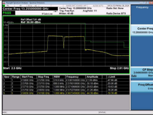
15MHz-20MHz_QPSK@QPSK-QPSK@QPSK_21179-21350_75RB#0@75RB#0-100RB#0@100RB#0
