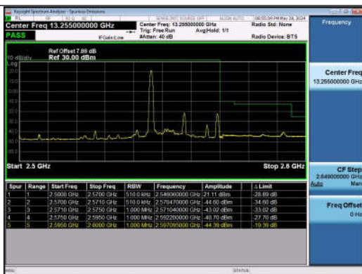
15MHz-10MHz_QPSK@QPSK-QPSK@QPSK_21277-21397_1RB#0@75RB#0-0RB#0@50RB#0
