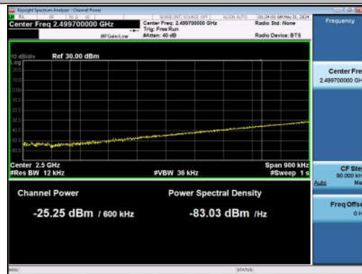
15MHz-15MHz_QPSK@QPSK-QPSK@QPSK_20825-20975_1RB#0@75RB#0-0RB#0@75RB#0_Final1
