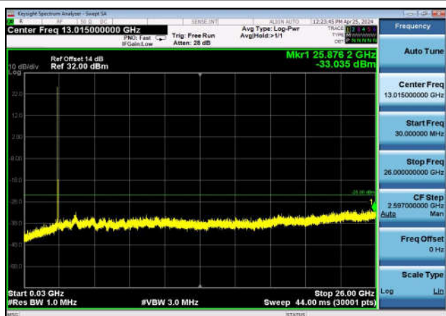
FDD07_LowRange_20MHz_30MHz~26GHz
