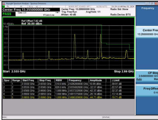
10MHz-20MHz_QPSK@QPSK-QPSK@QPSK_40996-41 140_1RB#0@50RB#0-1RB#99@100RB#0
