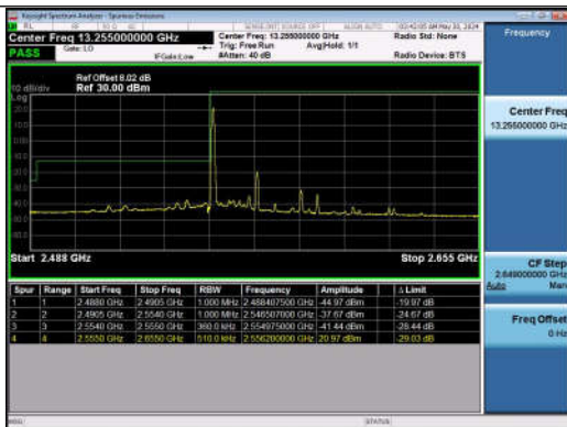
15MHz-20MHz_QPSK@QPSK-QPSK@QPSK_40318-40 489_1RB#0@75RB#0-0RB#0@100RB#0
