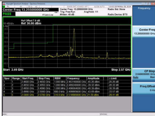
20MHz-15MHz_QPSK@QPSK-QPSK@QPSK_20850-2102 1_1RB#99@100RB#0-0RB#0@75RB#0
