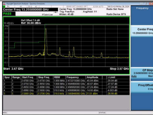
15MHz-10MHz_QPSK@QPSK-QPSK@QPSK_20825-209 45_1RB#0@75RB#0-0RB#0@50RB#0
