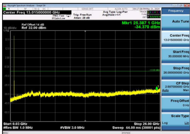
FDD17_LowRange_10MHz_30MHz~26GHz
