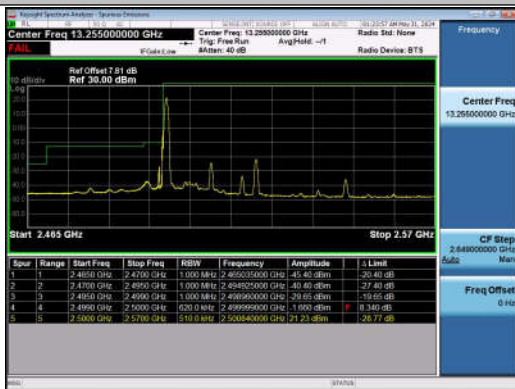
15MHz-15MHz_QPSK@QPSK-QPSK@QPSK_20825-20975_975_1RB#0@75RB#0-0RB#0@75RB#0
