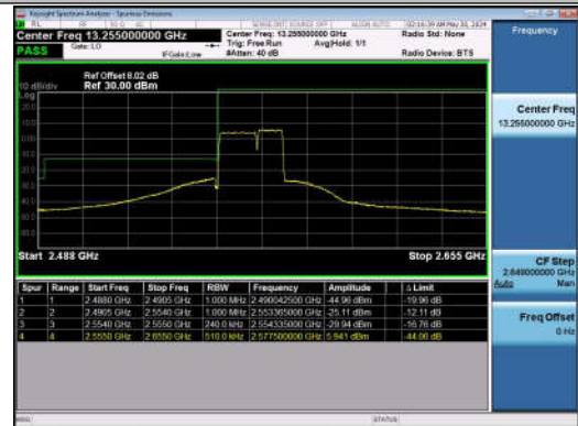
15MHz-10MHz_QPSK@QPSK-QPSK@QPSK_40315-40435 _75RB#0@75RB#0-50RB#0@50RB#0
