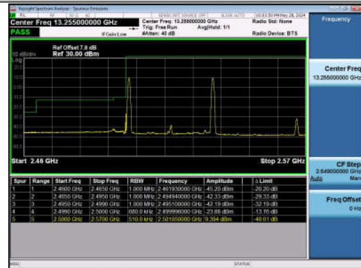
20MHz-15MHz_QPSK@QPSK-QPSK@QPSK_20850-210 21_1RB#0@100RB#0-1RB#74@75RB#0
