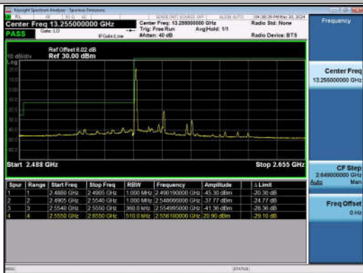
20MHz-15MHz_QPSK@QPSK-QPSK@QPSK_40340-40 511_1RB#0@100RB#0-0RB#0@75RB#0
