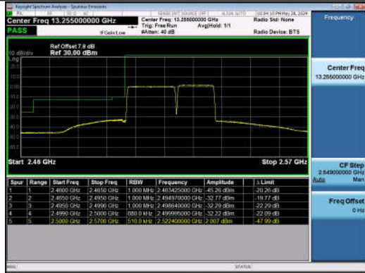
20MHz-15MHz_QPSK@QPSK-QPSK@QPSK_20850-2102_1_100RB#0@100RB#0-75RB#0@75RB#0
