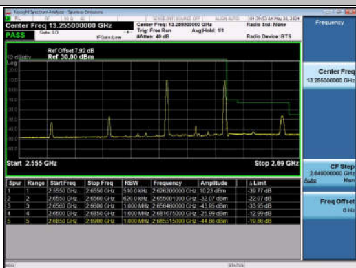
20MHz-10MHz_QPSK@QPSK-QPSK@QPSK_41041-41 185_1RB#0@100RB#0-1RB#49@50RB#0
