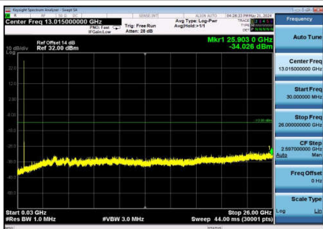
FDD17_MidRange_10MHz_30MHz~26GHz
