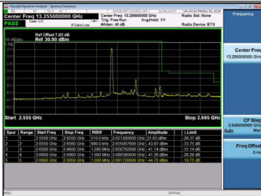
20MHz-15MHz_QPSK@QPSK-QPSK@QPSK_40991-41 162_1RB#0@100RB#0-0RB#0@75RB#0
