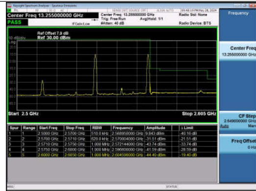
20MHz-10MHz_QPSK@QPSK-QPSK@QPSK_21251-213 95_1RB#0@100RB#0-1RB#49@50RB#0
