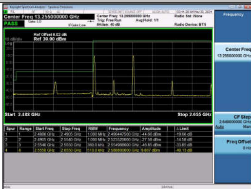
15MHz-20MHz_QPSK@QPSK-QPSK@QPSK_40318-40 489_1RB#0@75RB#0-1RB#99@100RB#0
