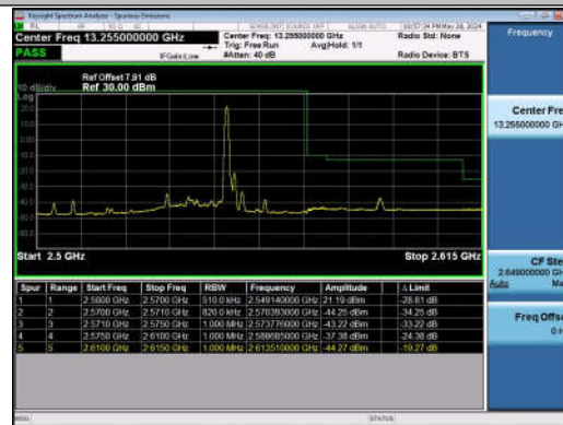
20MHz-20MHz_QPSK@QPSK-QPSK@QPSK_21152-21350_1RB#99@100RB#0-0RB#0@100RB#0
