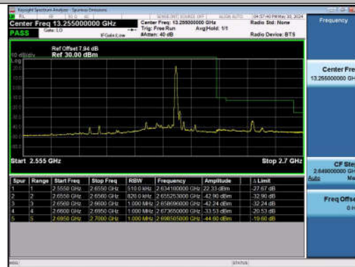
20MHz-20MHz_QPSK@QPSK-QPSK@QPSK_40942-41140 _1RB#99@100RB#0-0RB#0@100RB#0
