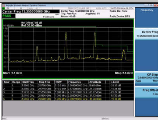
15MHz-10MHz_QPSK@QPSK-QPSK@QPSK_21277-21397_1RB#0@75RB#0-1RB#49@50RB#0
