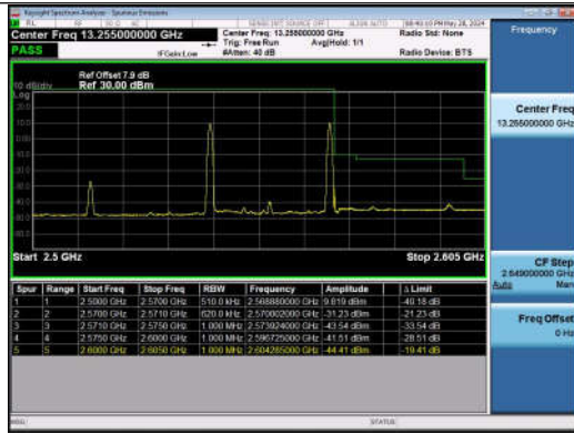
10MHz-20MHz_QPSK@QPSK-QPSK@QPSK_21206-213 50_1RB#0@50RB#0-1RB#99@100RB#0
