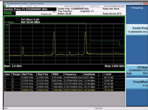
15MHz-15MHz_QPSK@QPSK-QPSK@QPSK_21225-213 75_1RB#0@75RB#0-1RB#74@75RB#0
