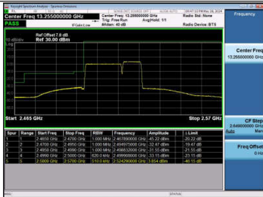
20MHz-10MHz_QPSK@QPSK-QPSK@QPSK_20850-20994_100RB#0@100RB#0-50RB#0@50RB#0
