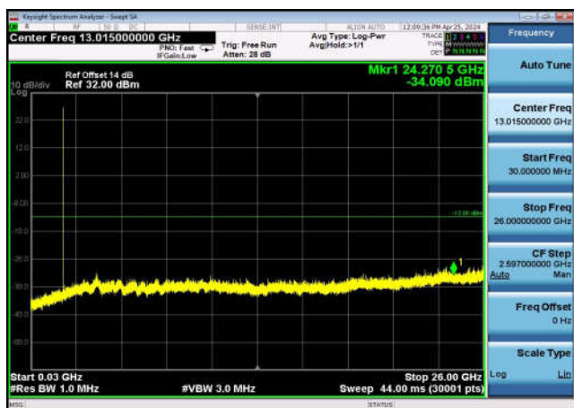
FDD02_MidRange_20MHz_30MHz~26GHz
