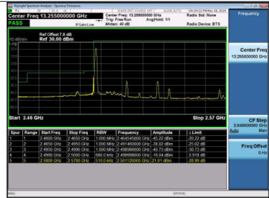
15MHz-20MHz_QPSK@QPSK-QPSK@QPSK_20828-209 99_1RB#0@75RB#0-0RB#0@100RB#0
