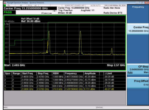
15MHz-15MHz_QPSK@QPSK-QPSK@QPSK_20825-209 75_1RB#0@75RB#0-1RB#74@75RB#0
