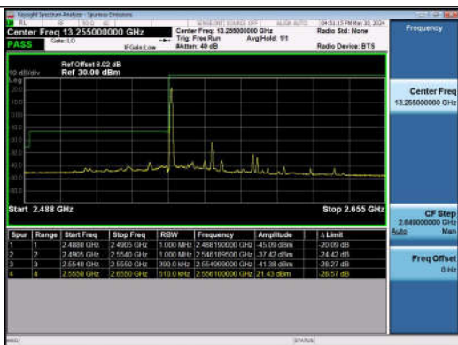
20MHz-20MHz_QPSK@QPSK-QPSK@QPSK_40340-40 538_1RB#0@100RB#0-0RB#0@100RB#0
