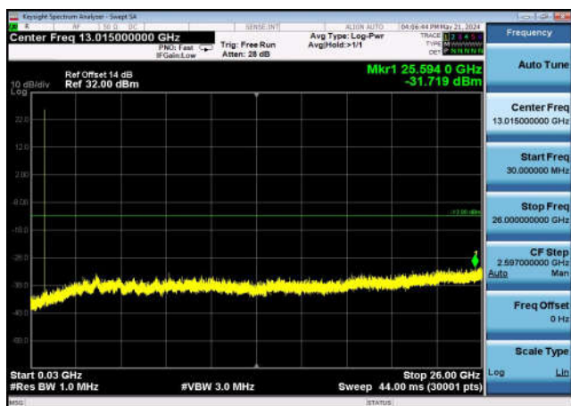
FDD07_HighRange_20MHz_30MHz~26GHz
