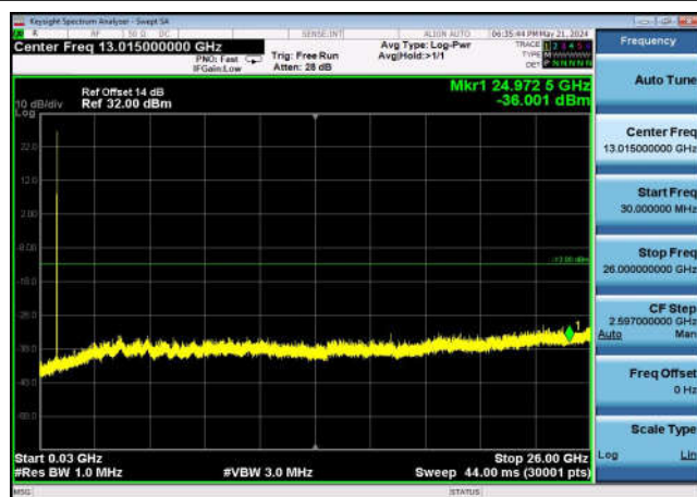
FDD26_Part 22_MidRange_15MHz_30MHz~26GHz
