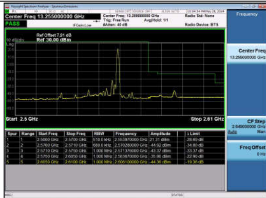
20MHz-15MHz_QPSK@QPSK-QPSK@QPSK_21201-2137_2_1RB#99@100RB#0-0RB#0@75RB#0
