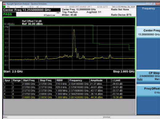
15MHz-15MHz_QPSK@QPSK-QPSK@QPSK_21225-2137 5_1RB#74@75RB#0-0RB#0@75RB#0
