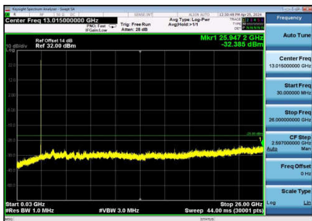
FDD07_MidRange_20MHz_30MHz~26GHz
