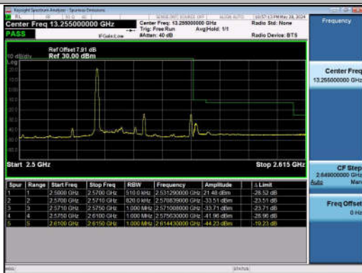
20MHz-20MHz_QPSK@QPSK-QPSK@QPSK_21152-21350_350_1RB#0@100RB#0-0RB#0@100RB#0
