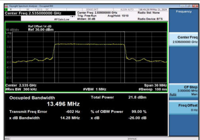
FDD07_MidRange_15_2535_QPSK
