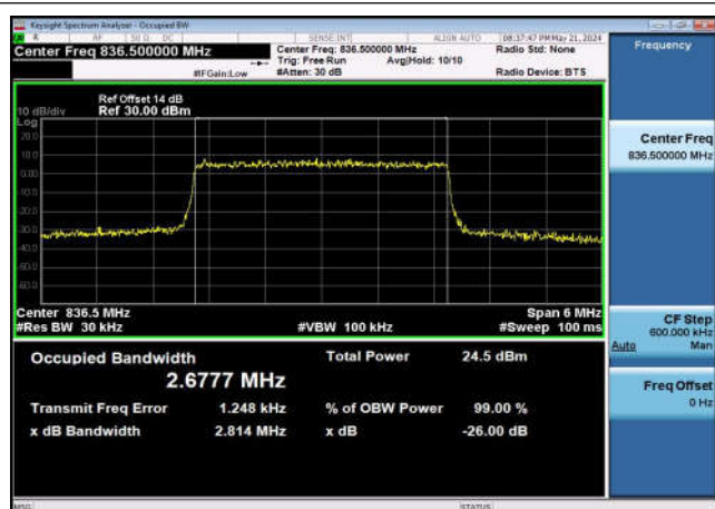
FDD05_MidRange_3_836.5_QPSK
