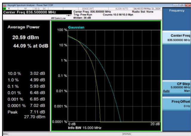
FDD26_Part 22_MidRange_15MHz_836.5_fullIRB_Q16
