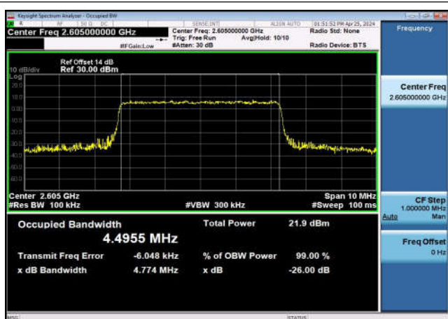
TDD41_MidRange_5_2605_Q16
