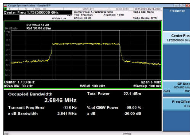
FDD04_MidRange_5_1732.5_QPSK
