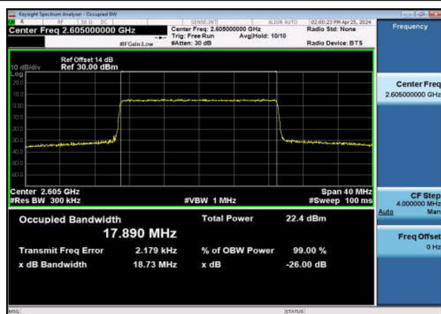
TDD41_MidRange_5_2605_QPSK
