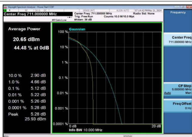
FDD17_LowRange_10MHz_709_OneRB _high_Q16
