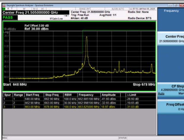
Band71_15MHz_QPSK_133197_1RB#0
