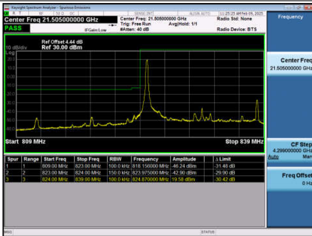
Band26_15MHz_QPSK_26965_1RB#74
