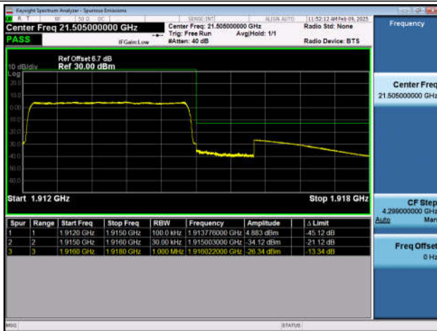
Band25_5MHz_QPSK_26065_25RB#0
