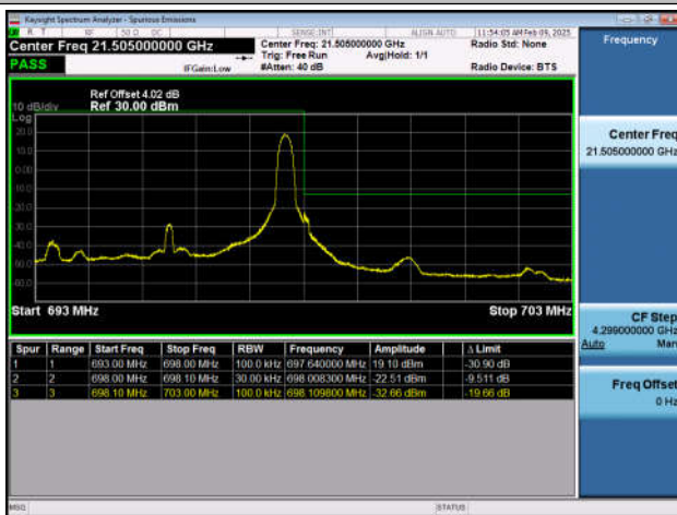
Band71_5MHz_QPSK_133447_1RB#24
