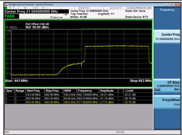
Band71_20MHz_QPSK_133372_100RB#0
