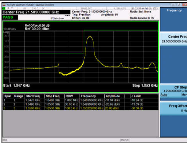
Band25_3MHz_QPSK_26055_15RB#0
