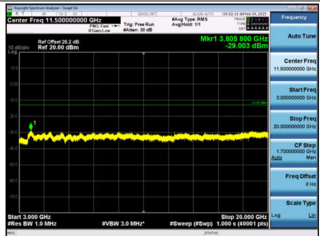
Band4_20MHz_QPSK_20050_1RB#0_3000~20000_3000~20000
