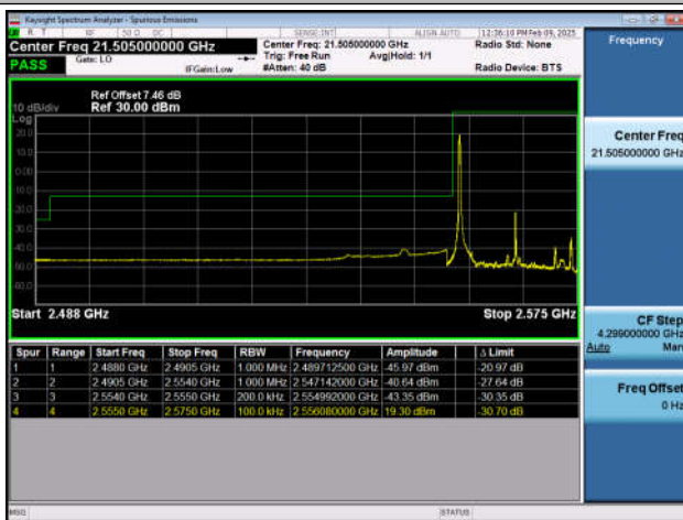
Band41_20MHz_QPSK_40340_1RB#0
