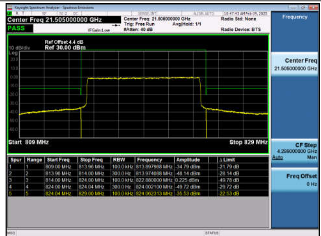
Band26_1.4MHz_QPSK_26797_6RB#0
