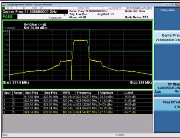
Band26_3MHz_QPSK_26705_15RB#0
