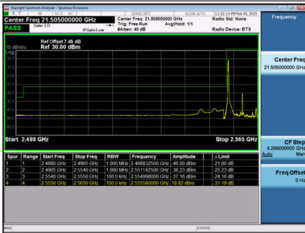
Band41_10MHz_QPSK_41190_1RB#49
