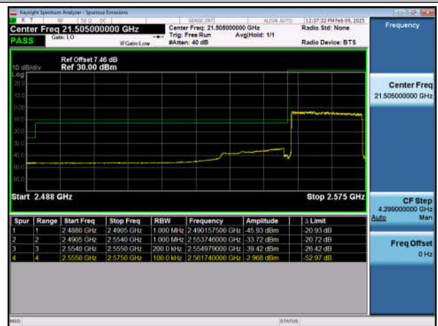
Band41_20MHz_QPSK_40340_100RB#0
