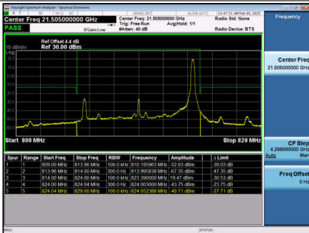
Band26_1.4MHz_QPSK_26797_1RB#0
