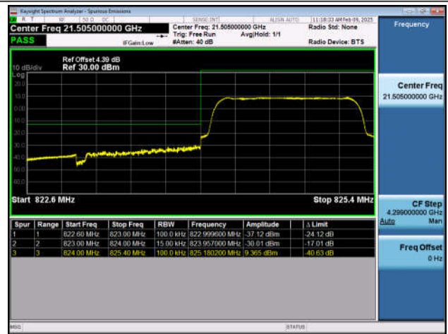
Band26_1.4MHz_QPSK_27033_6RB#0
