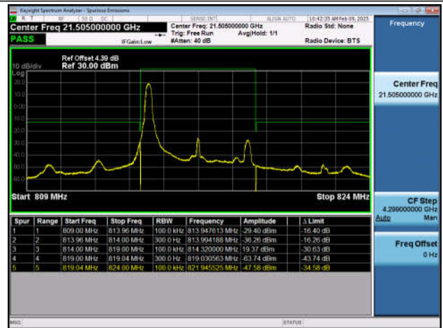
Band26_5MHz_QPSK_26765_1RB#24
