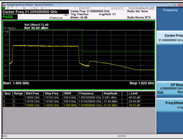
Band25_15MHz_QPSK_26115_75RB#0
