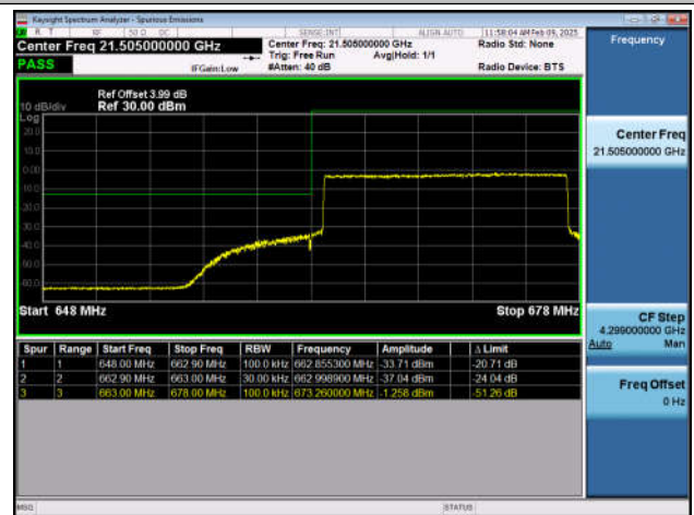
Band71_15MHz_QPSK_133197_75RB#0
