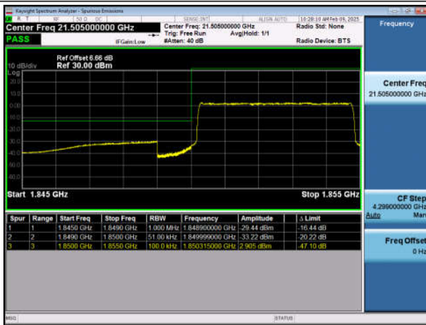
Band25_5MHz_QPSK_26665_25RB#0
