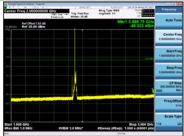
Band2_20MHz_QPSK_19100_1RB#0_1000~3000_1000~3000
