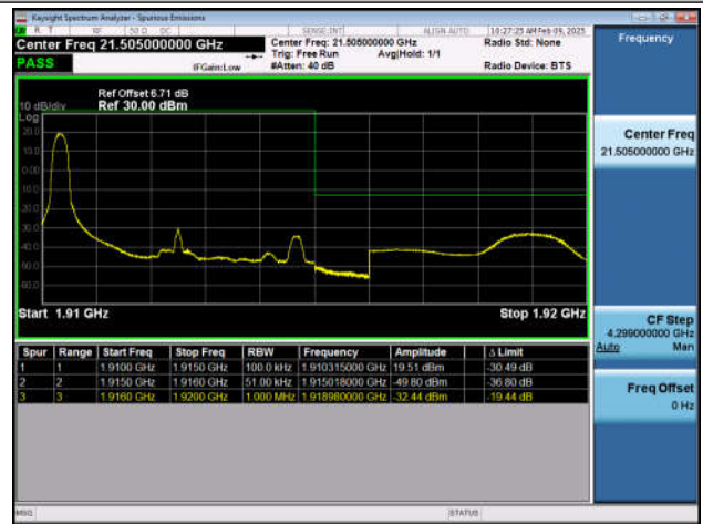
Band25_10MHz_QPSK_26090_1RB#0
