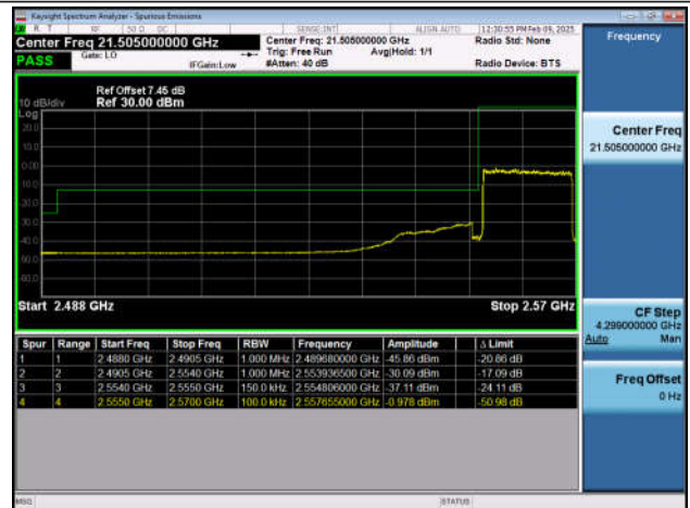
Band41_15MHz_QPSK_41165_75RB#0
