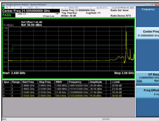
Band41_5MHz_QPSK_40265_1RB#0
