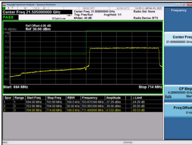
Band17_10MHz_QPSK_23800_50RB#0
