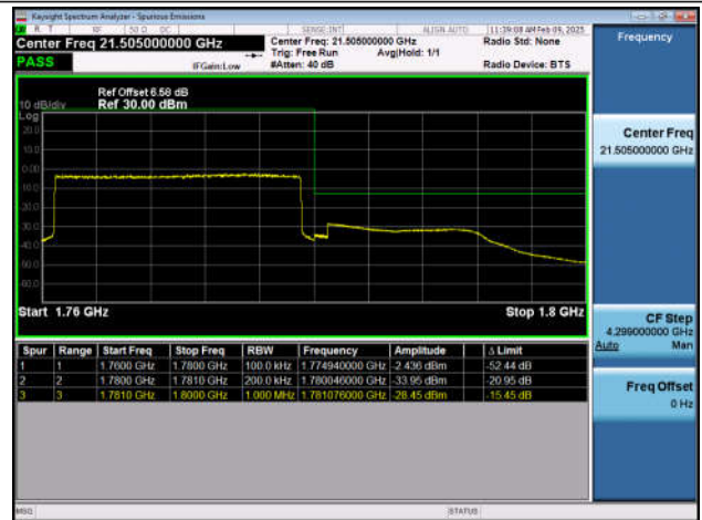
Band71_5MHz_QPSK_133147_25RB#0
