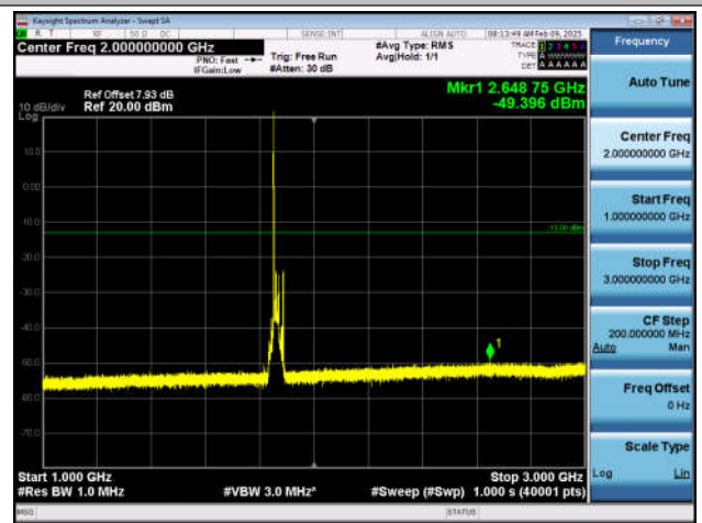
Band2_20MHz_QPSK_18700_1RB#0_1000~3000_1000~3000
