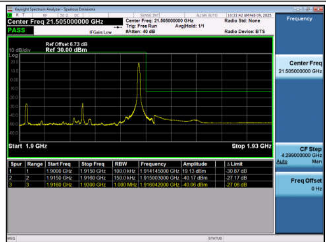
Band25_15MHz_QPSK_26615_1RB#74
