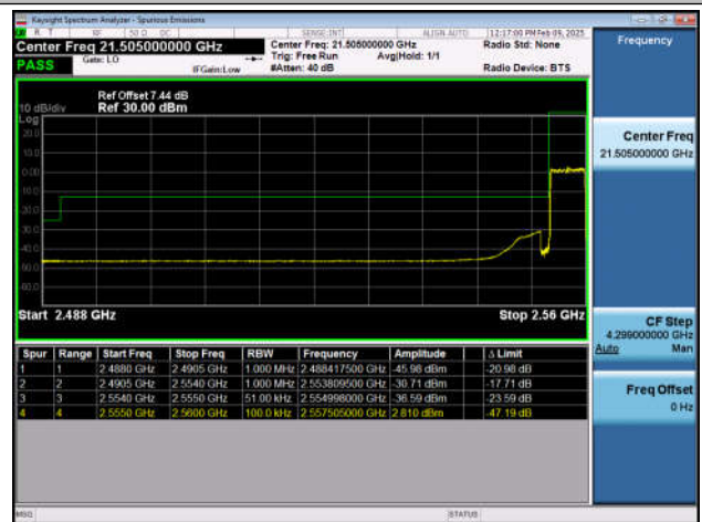
Band41_5MHz_QPSK_40265_25RB#0
