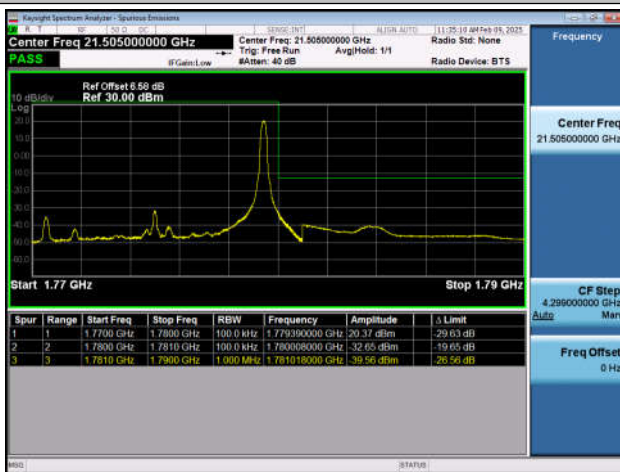
Band66_10MHz_QPSK_132622_1RB#49
