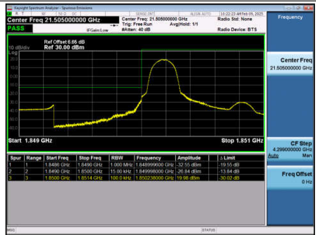
Band25_1.4MHz_QPSK_26047_6RB#0
