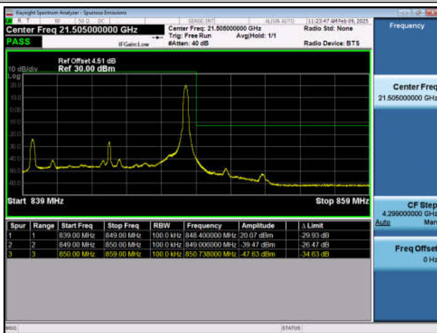
Band26_10MHz_QPSK_26990_1RB#49
