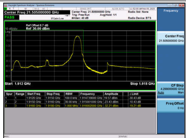
Band25_3MHz_QPSK_26675_1RB#14
