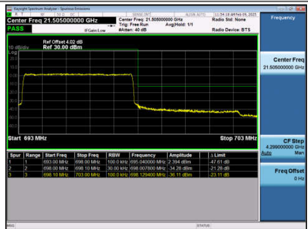
Band71_5MHz_QPSK_133447_25RB#0
