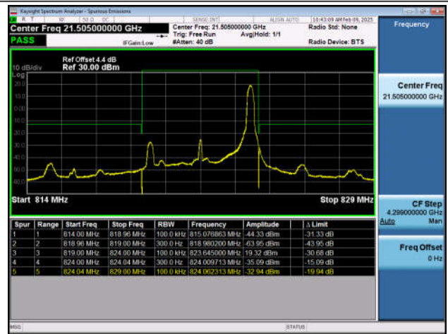
Band26_10MHz_QPSK_26740_1RB#0
