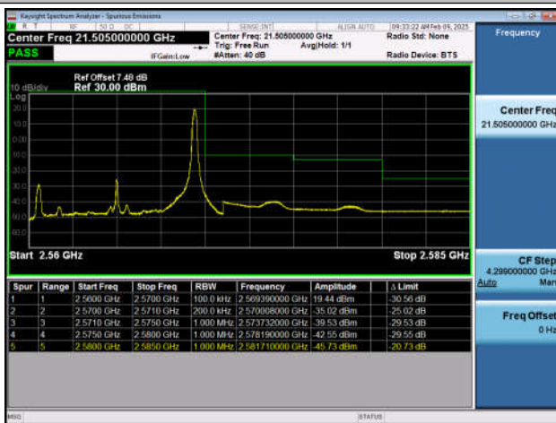
Band7_10MHz_QPSK_21400_1RB#49
