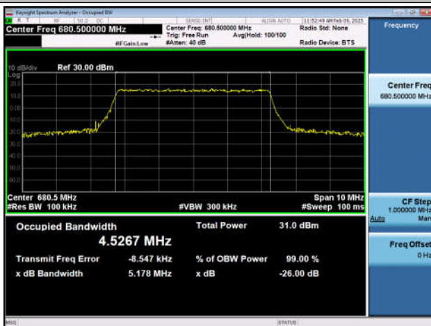
Band71-5MHz-QPSK-133297-25RB#0-PASS
