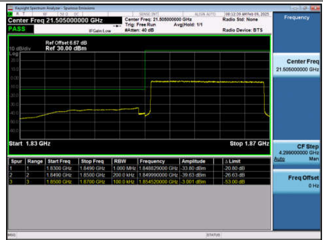
Band2_20MHz_QPSK_19100_100RB#0
