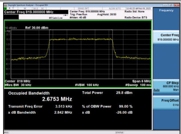
Band26(814-824)-3MHz-16QAM-26740-15RB#0-PASS
