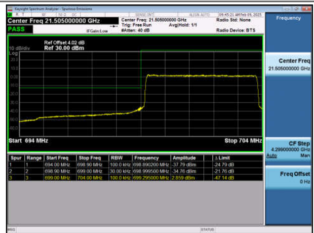
Band12_5MHz_QPSK_23035_25RB#0
