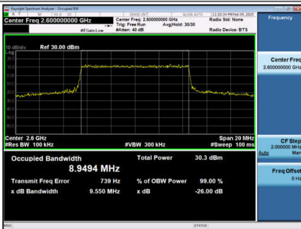
Band41-10MHz-QPSK-40690-50RB#0-PASS
