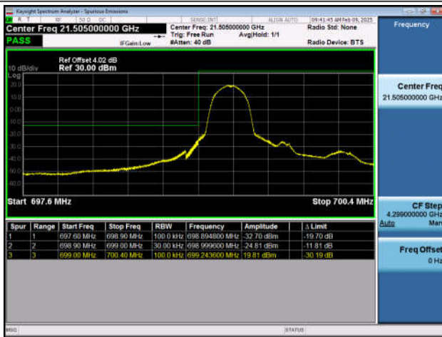
Band12_1.4MHz_QPSK_23173_1RB#5
