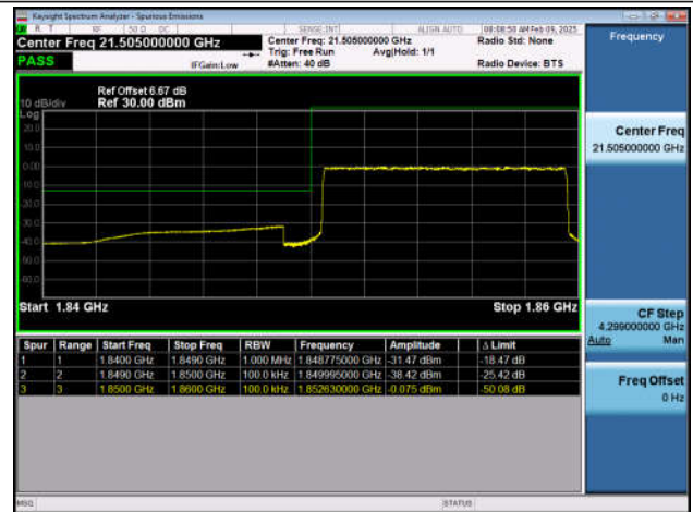
Band2_10MHz_QPSK_19150_50RB#0
