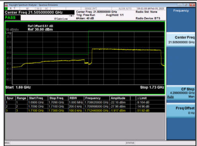
Band4_20MHz_QPSK_20300_100RB#0
