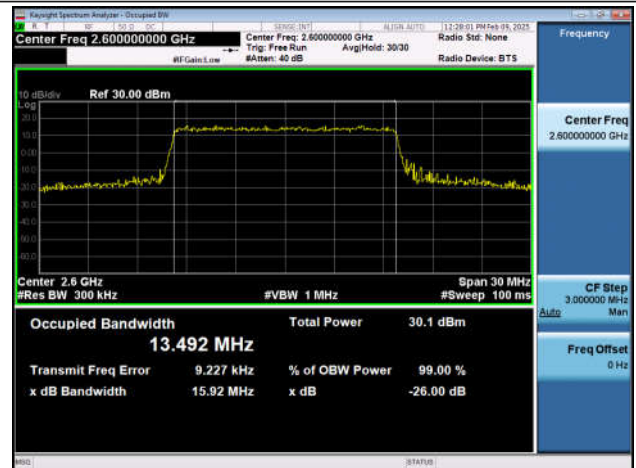
Band41-20MHz-16QAM-40690-100RB#0-PASS
