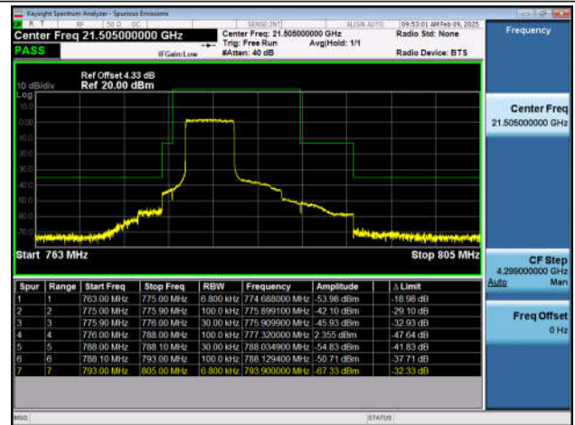
Band13_5MHz_QPSK_23255_25RB#0
