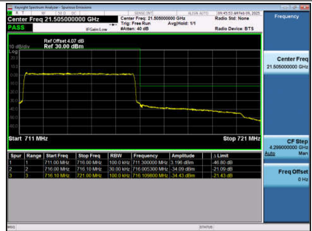
Band12_10MHz_QPSK_23060_50RB#0
