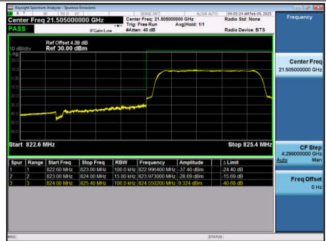
Band5_1.4MHz_QPSK_20643_6RB#0
