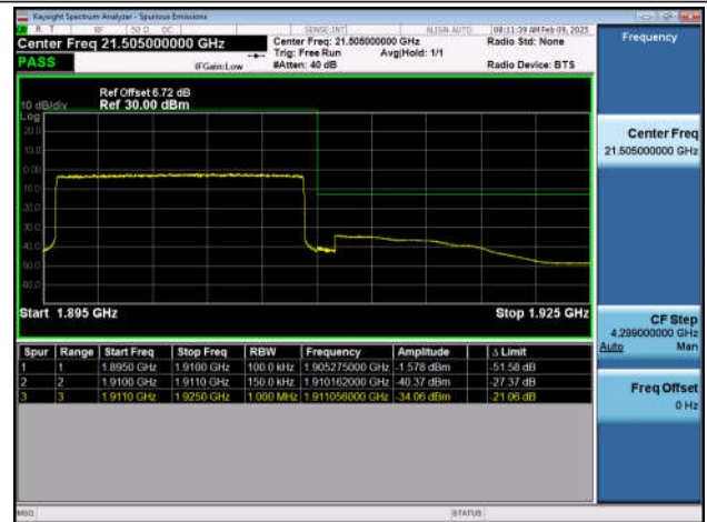
Band2_20MHz_QPSK_18700_100RB#0
