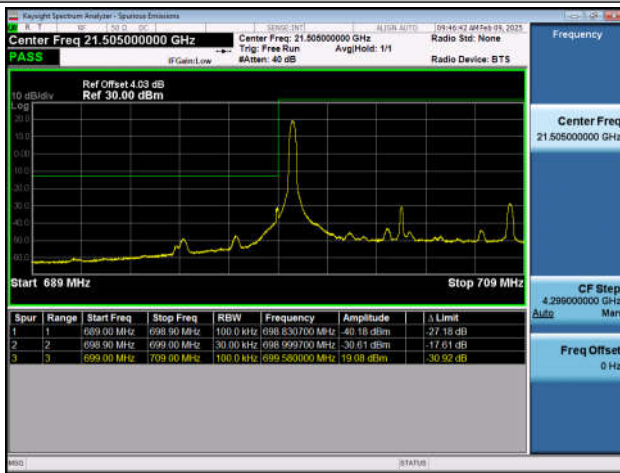
Band12_10MHz_QPSK_23130_1RB#49
