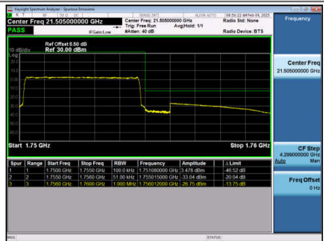
Band4_5MHz_QPSK_20375_25RB#0
