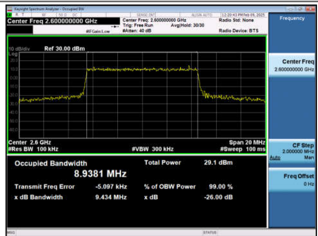
Band41-10MHz-16QAM-40690-50RB#0-PASS
