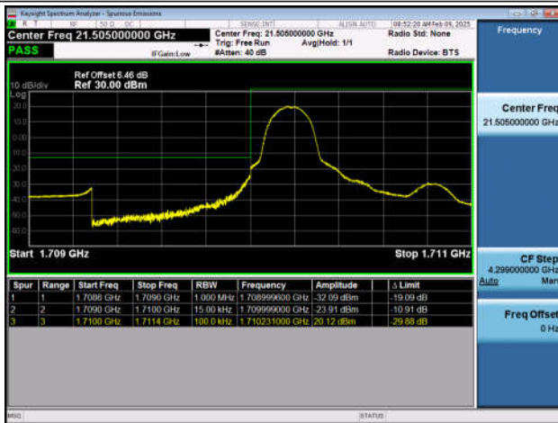
Band4_1.4MHz_QPSK_20393_1RB#5
