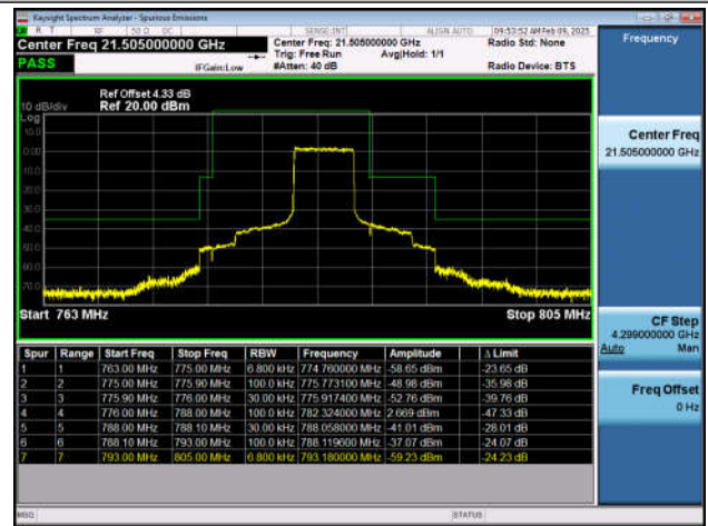
Band13_10MHz_QPSK_23230_1RB#49
