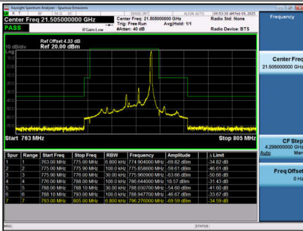
Band13_10MHz_QPSK_23230_1RB#0
