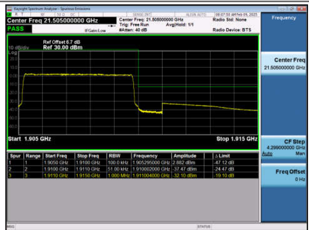
Band2_5MHz_QPSK_19175_25RB#0
