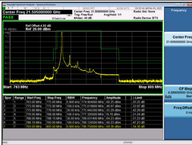
Band13_5MHz_QPSK_23255_1RB#24
