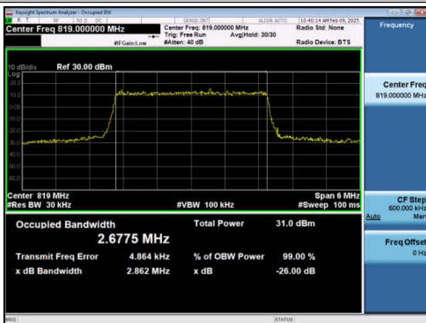
Band26(814-824)-3MHz-QPSK-26740-15RB#0-PASS
