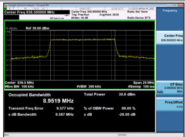
Band26(824-849)-10MHz-16QAM-26915-50RB#0-PASS
