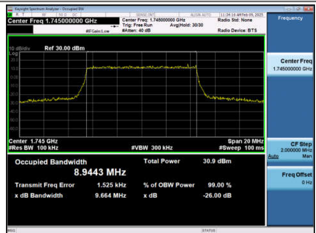
Band66-10MHz-16QAM-132322-50RB#0-PASS
