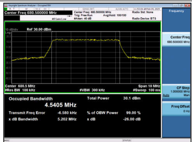
Band71-5MHz-16QAM-133297-25RB#0-PASS
