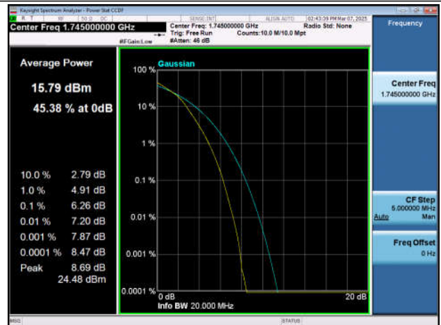
Band66-20MHz-16QAM-132572-100RB#0-PASS
