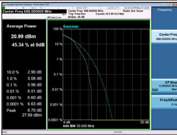
Band71-20MHz-16QAM-133372-1RB#0-PASS
