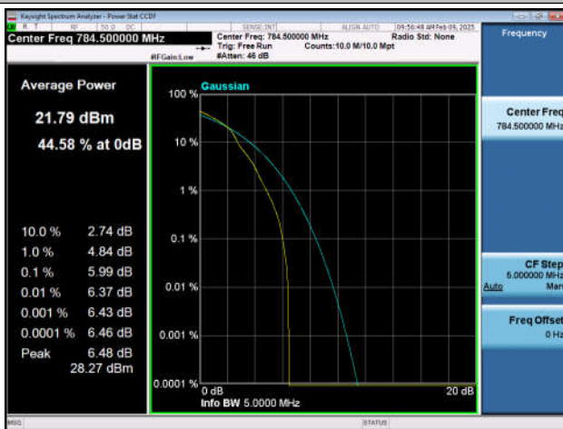
Band13-5MHz-16QAM-23255-1RB#0-PASS
