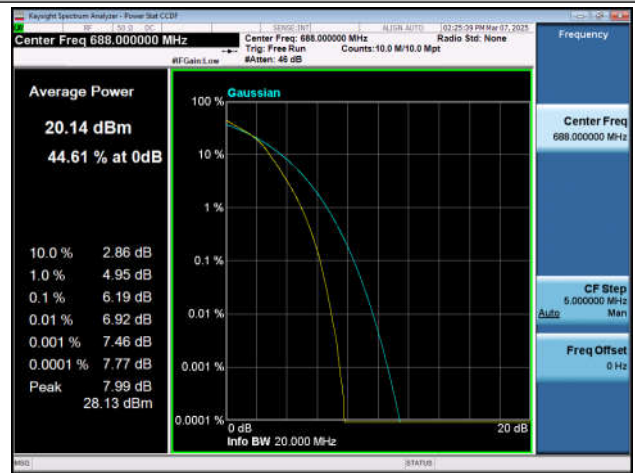
Band71-20MHz-16QAM-133372-100RB#0-PASS
