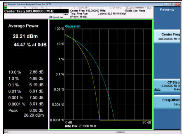
Band71-20MHz-16QAM-133372-100RB#0-PASS
