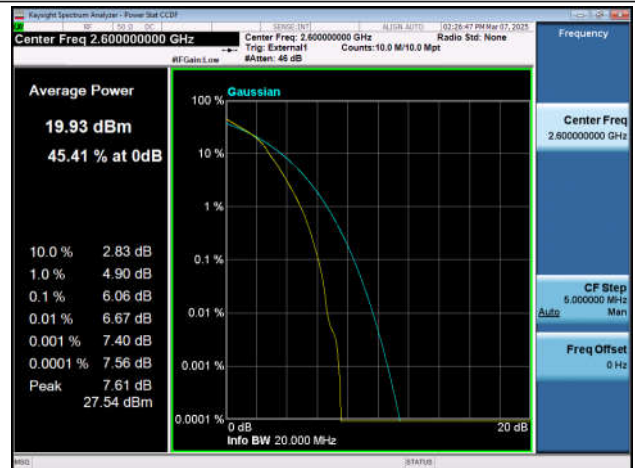
Band41-20MHz-16QAM-41140-100RB#0-PASS
