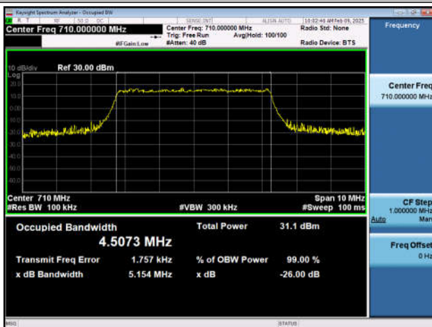
Band17-5MHz-QPSK-23790-25RB#0-PASS
