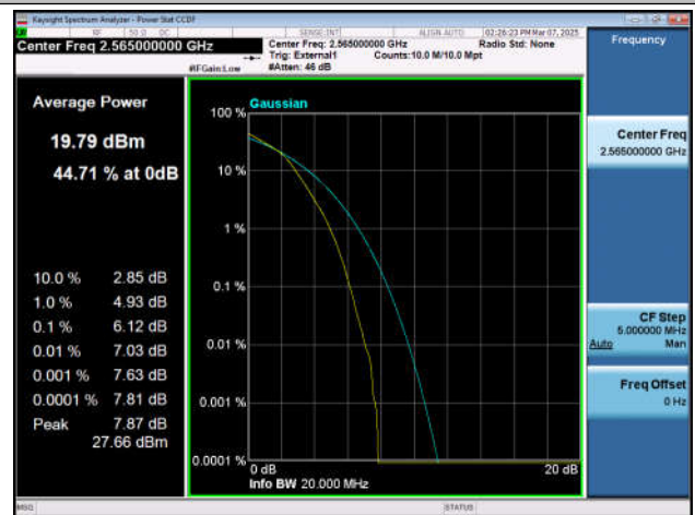
Band41-20MHz-16QAM-40340-100RB#0-PASS
