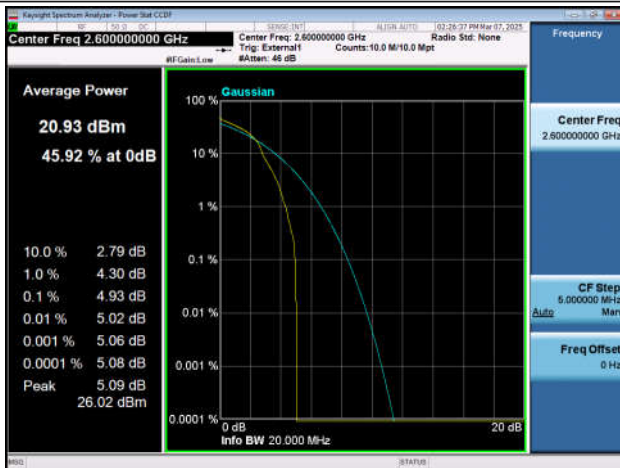
Band41-20MHz-16QAM-41140-1RB#0-PASS
