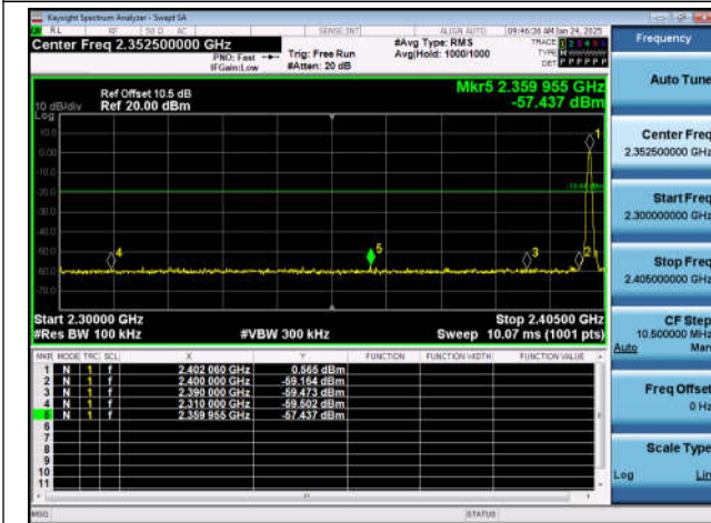
DH5-Ant1-Hop_2402-PASS
