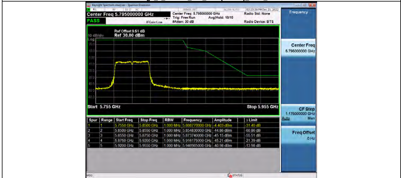
Bandedge_5_8WiFi_802_11ac(VHT40)_5795_40M
