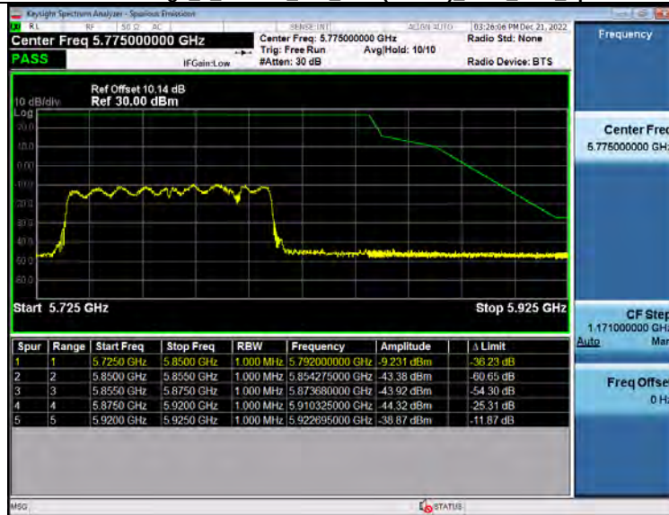
Bandedge 5 8GWiFi 802_11ac(VHT80) 5775 80M up
