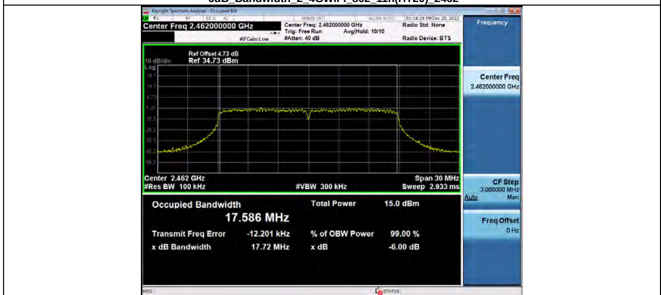
-6dB_Bandwidth_2_4GWiFi_802_11n(HT20)_2462
