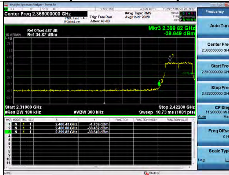
2_Bandedge_2_4GWiFi_NVNT_ANT1_802_11g_2412
