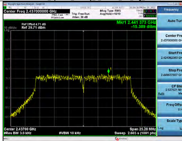
Power_Spectral_Density_2_4GWiFi_802_11g_2437
