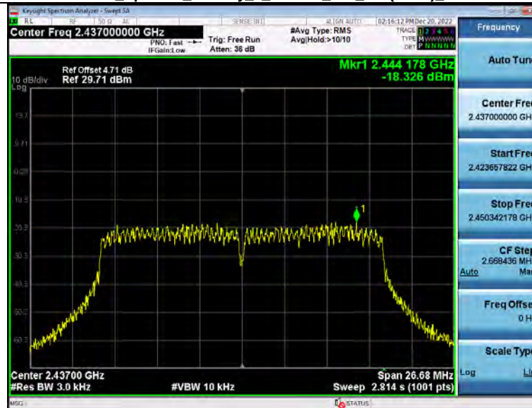
Power Spectral Density 2_4GWiFi_802_11n(HT20)_2437
