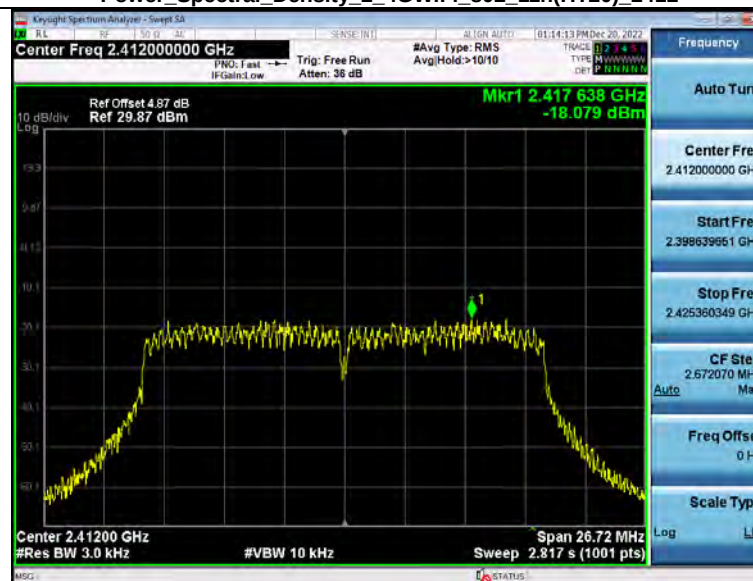
Power_Spectral_Density_2_4GWiFi_802_11n(HT20)_2412
