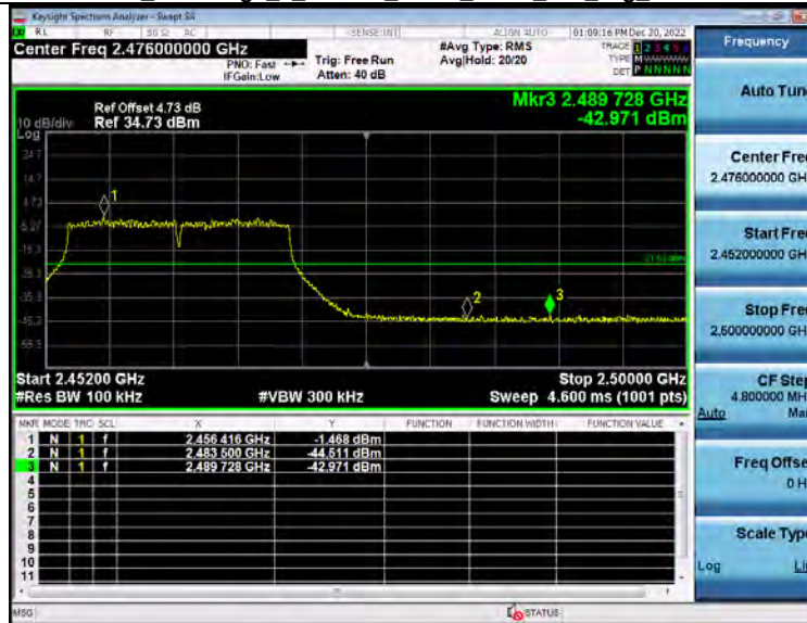
2_Bandedge_2_4GWiFi_NVNT_ANT1_802_11g_2462
