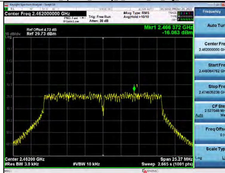
Power_Spectral_Density_2_4GWiFi_802_11g_2462
