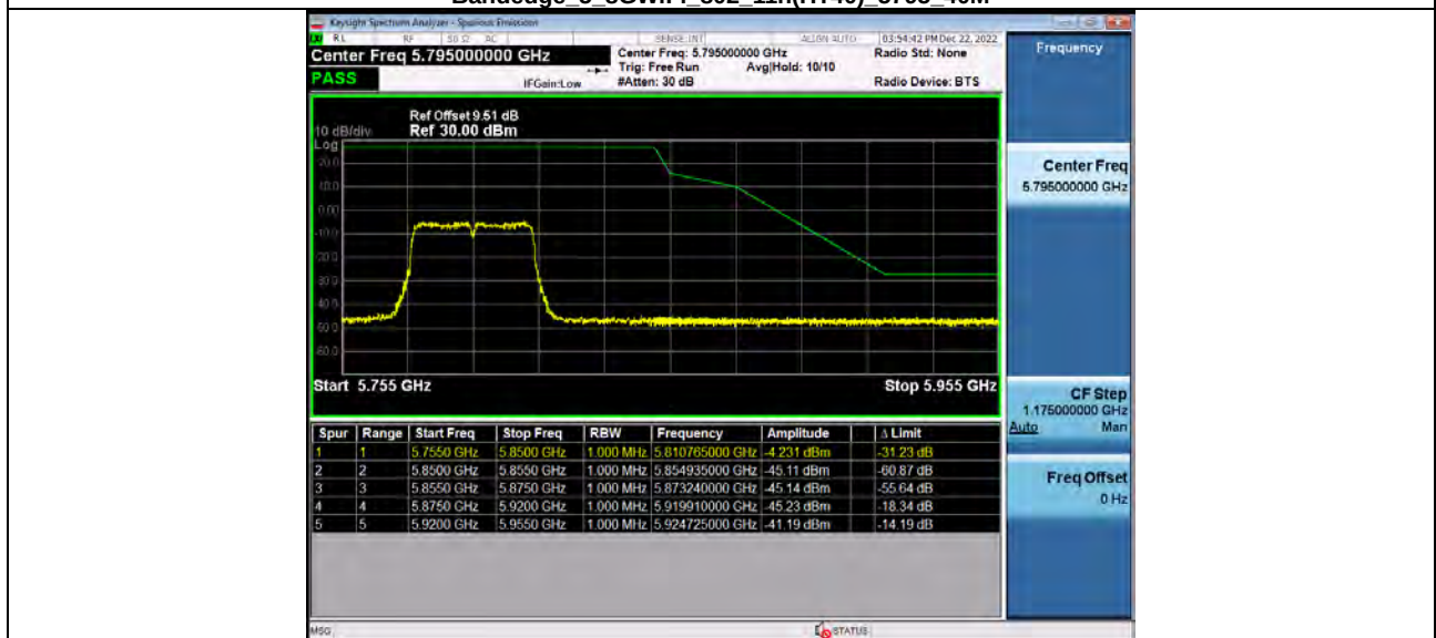
Bandedge_5_8WiFi_802_11n(HT40)_5795_40M
