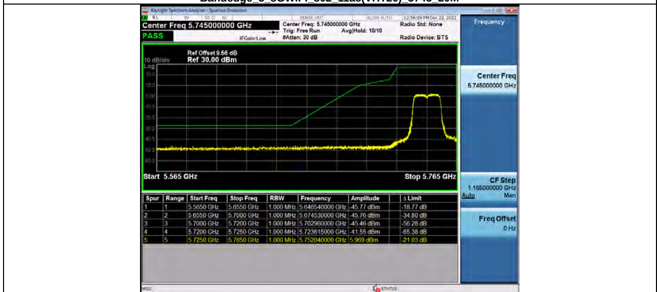
Bandedge_5_8WiFi_802_11ac(VHT20)_5745_20M
