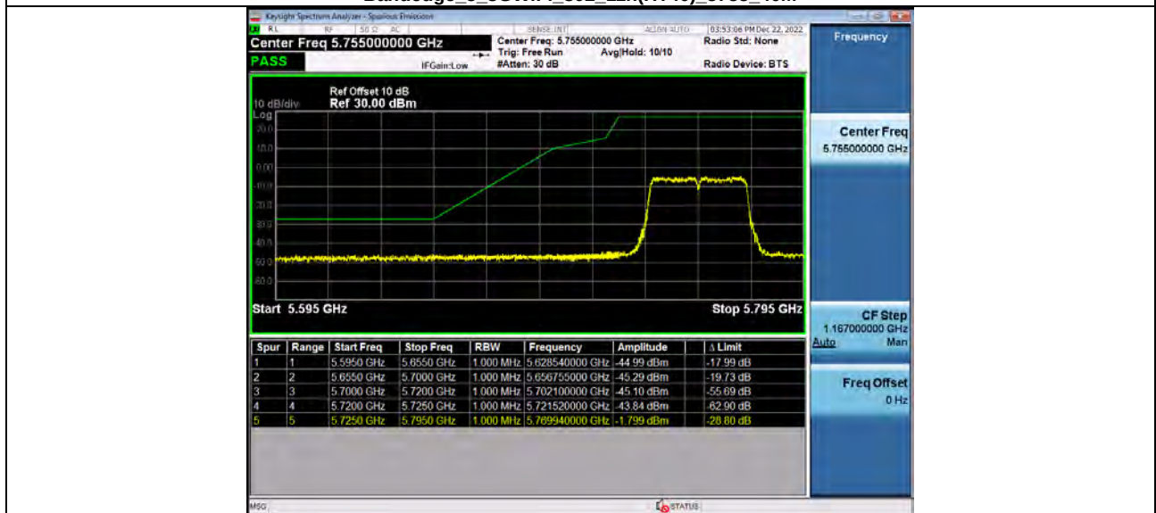
Bandedge_5_8WiFi_802_11n(HT40)_5755_40M
