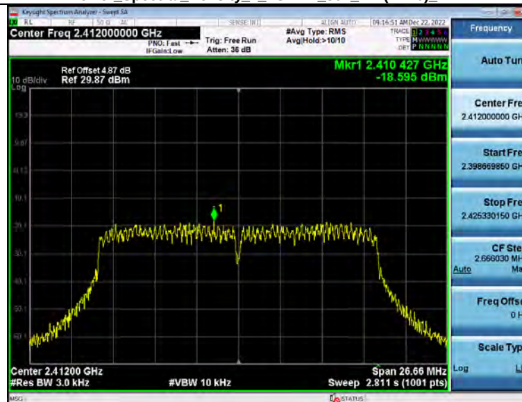
Power Spectral Density 2_4GWiFi_802_11n(HT20)_2412
