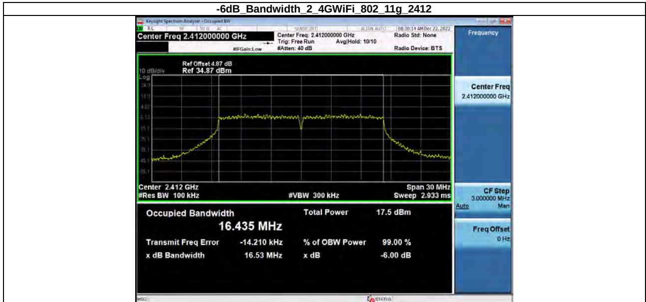
-6dB_Bandwidth_2_4GWiFi_802_11g_2412
