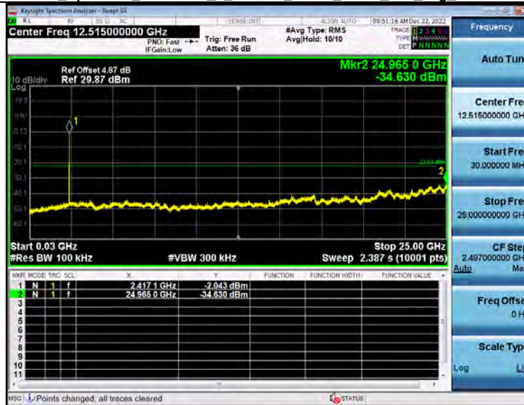
2 Spurious Emission 2_4GWiFi_NVNT_ANT1_802_11g_2412
