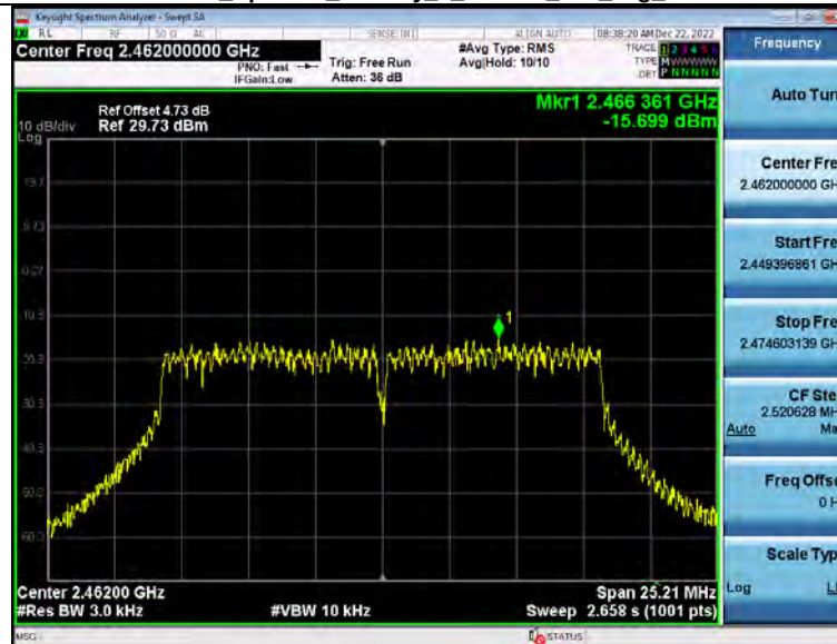
Power Spectral Density 2_4GWiFi_802_11g_2462
