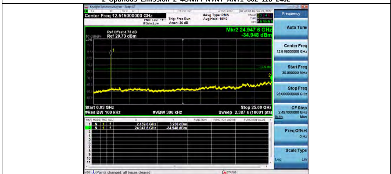
2 Spurious Emission 2 4GWiFi_NVNT_ANT1 802_11b 2462
