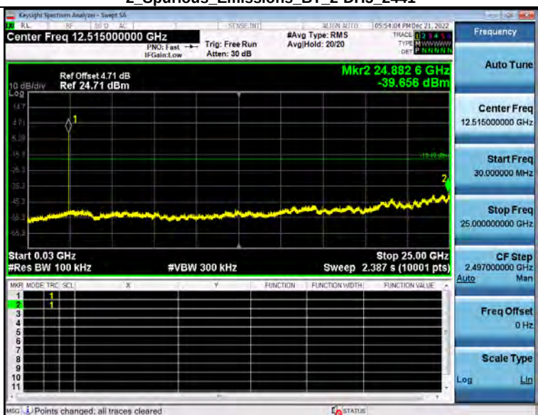
2_Spurious Emissions_BT 2-DH5_2441
