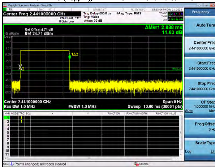
Dwell_Time (Hopping)_BT_1-DH5_2441_One_Burst_Time
