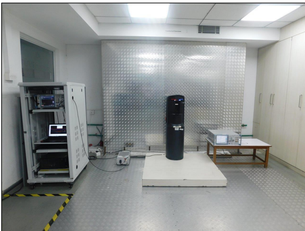
Conducted emission AC power lines test setup
