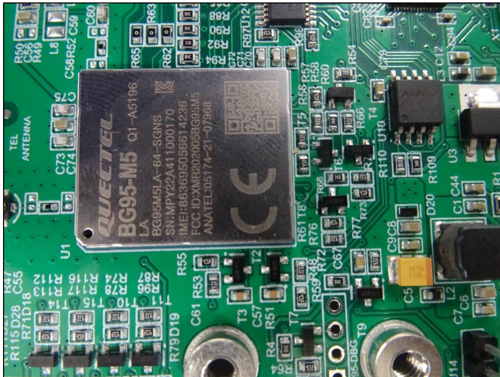
Figure 5: Module View
