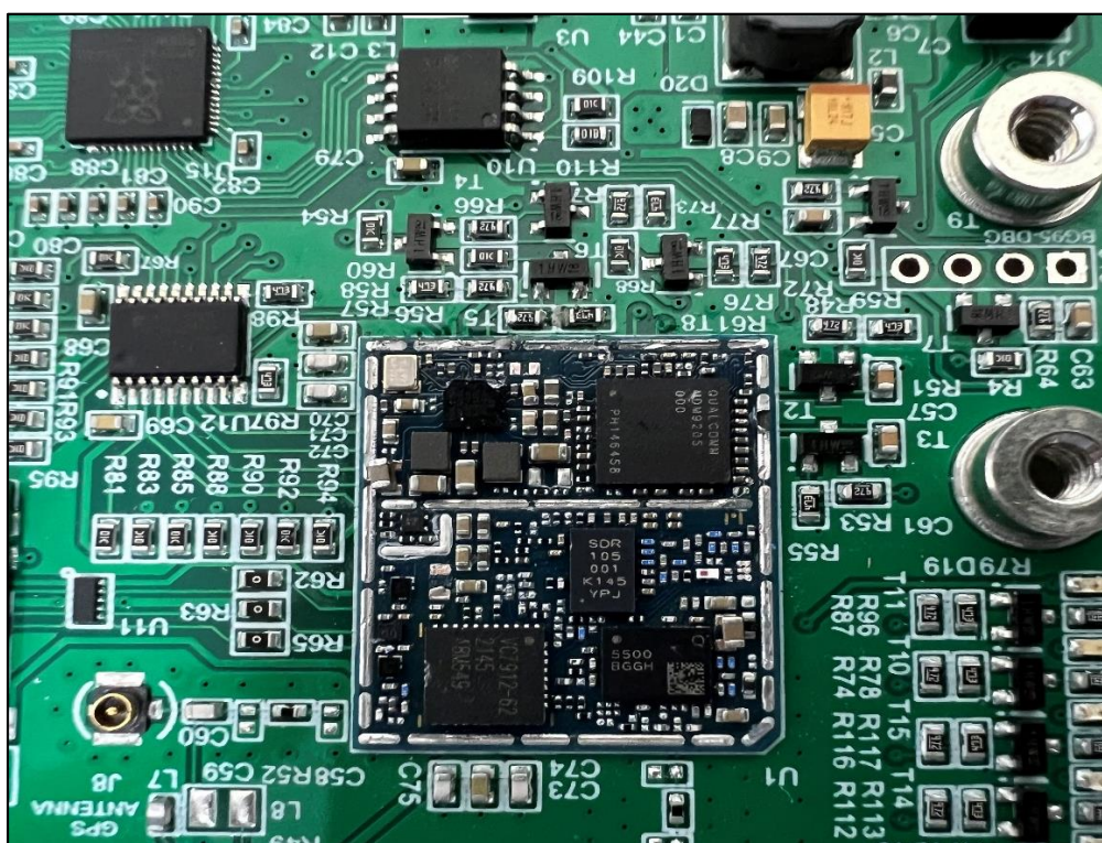
Figure 6: Without Shielding View
