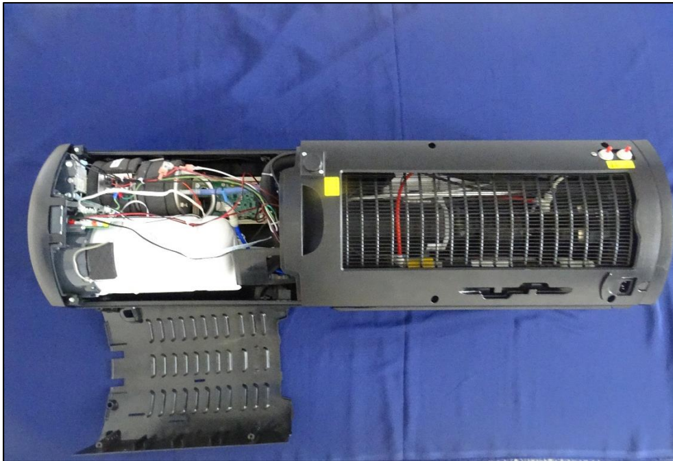
Figure 3: EUT with enclosure open view
