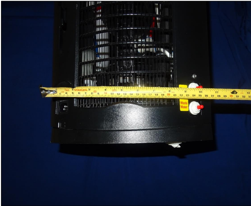
Figure 5: Dimensional view of the EUT
