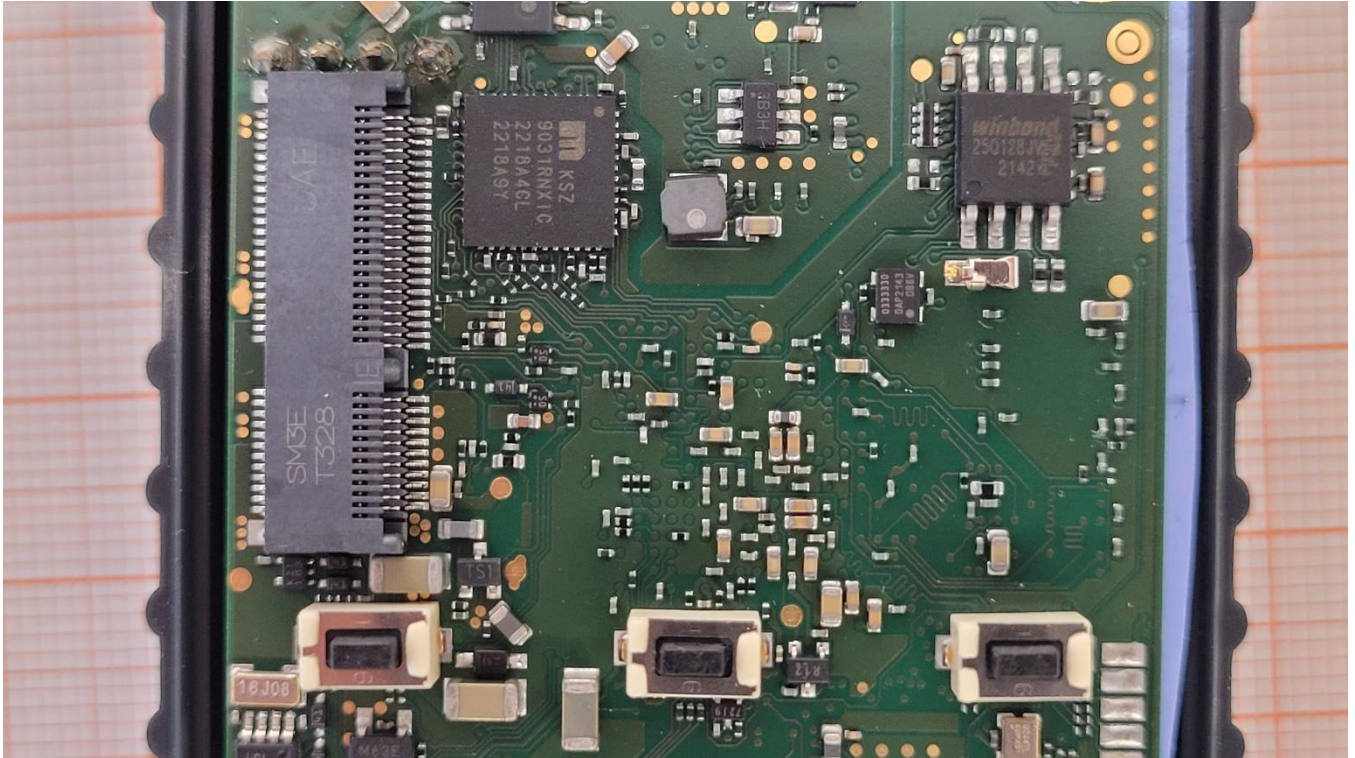
Photo No. 16: radiated test sample
