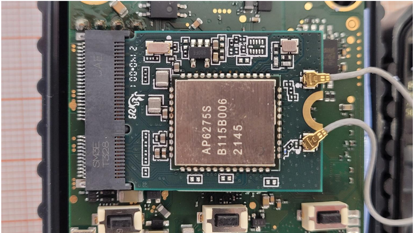
Photo No. 12: radiated test sample
