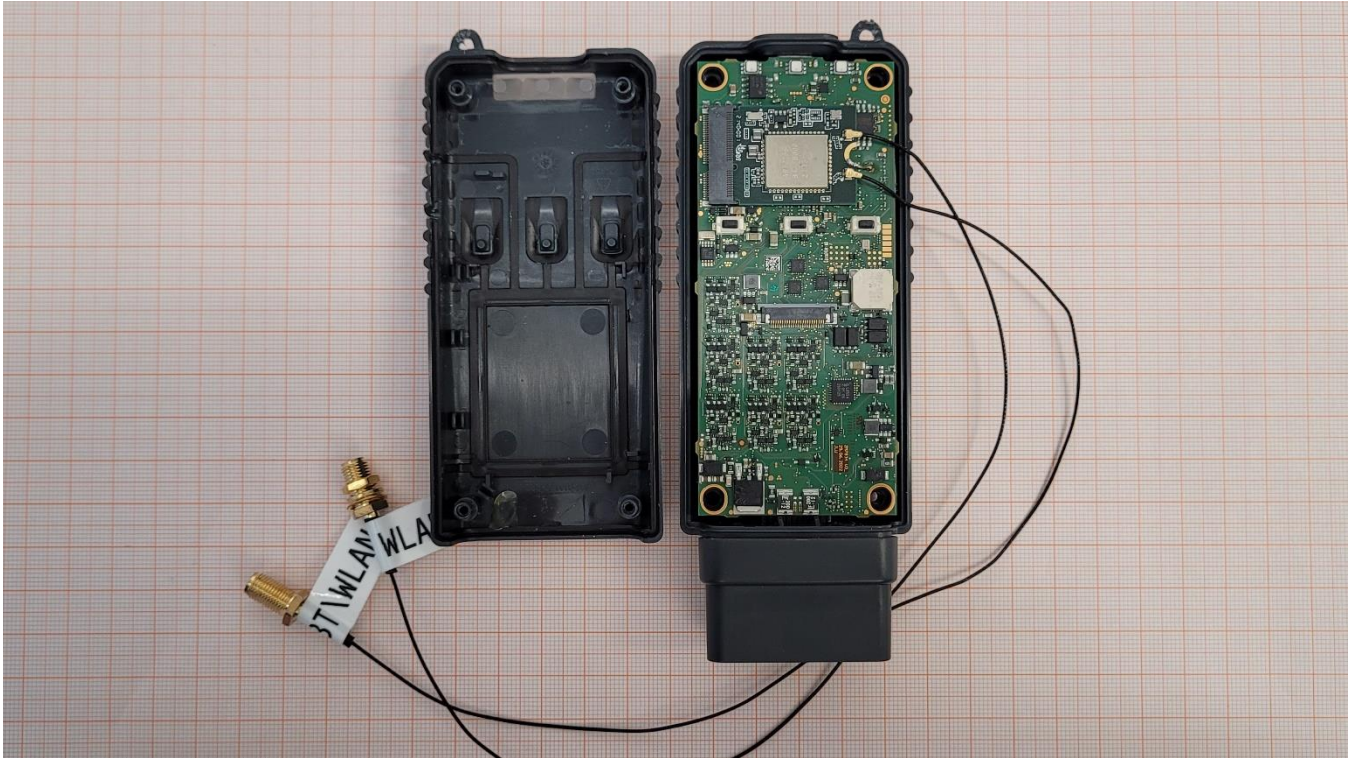
Photo No. 22: conducted test sample
