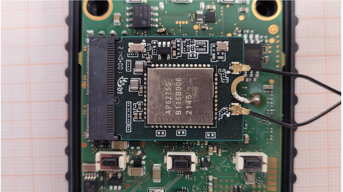
Photo No. 24: conducted test sample
