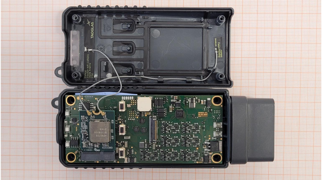
Photo No. 8: radiated test sample
