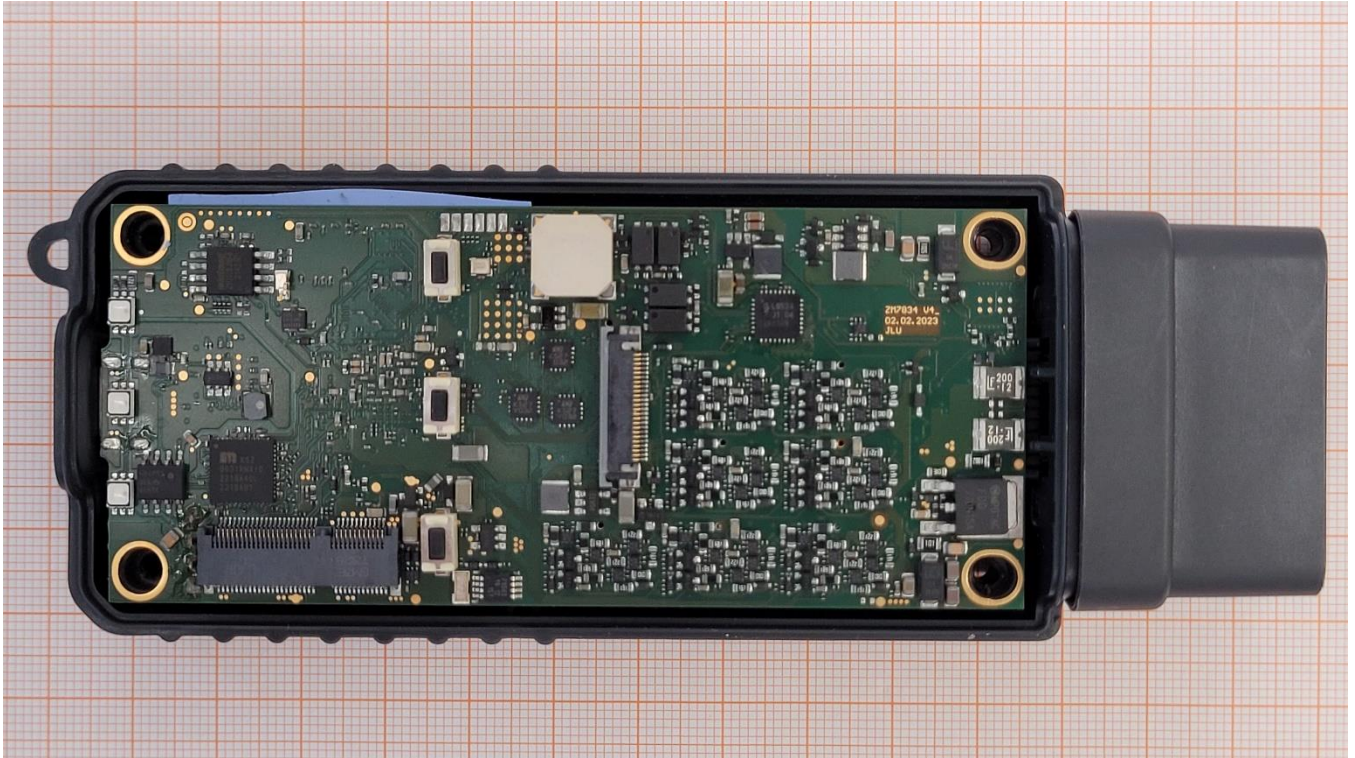
Photo No. 14: radiated test sample
