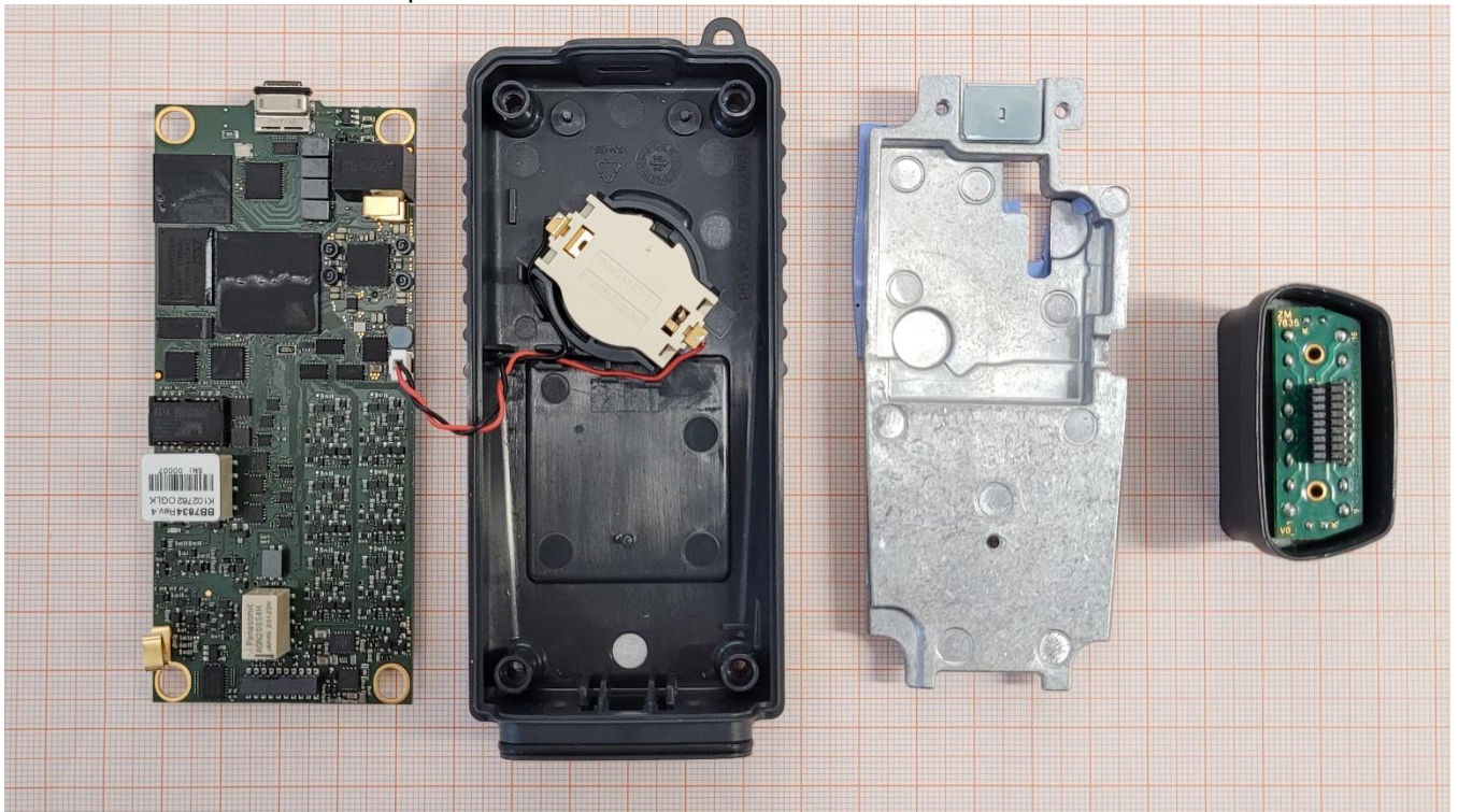
Photo No. 21: radiated test sample
