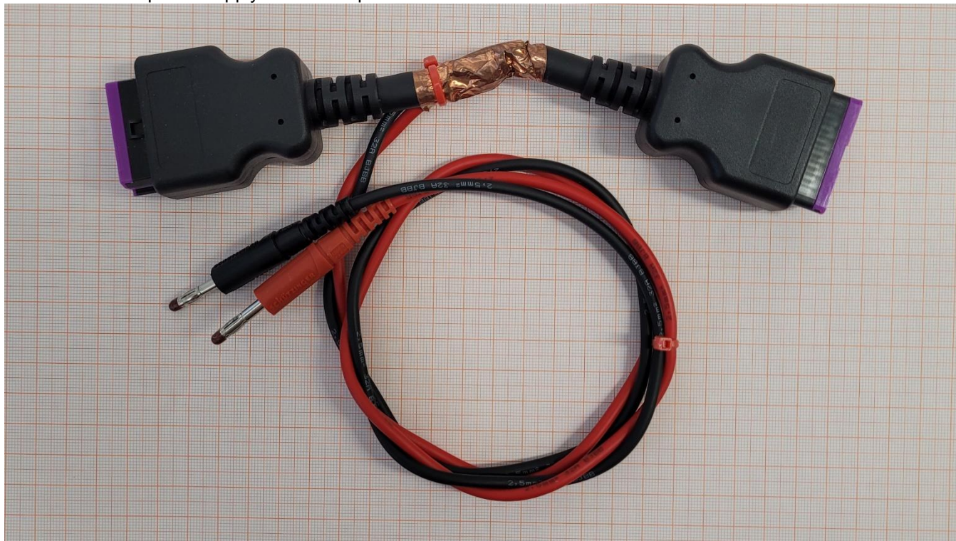
Photo No. 7: DC power supply cable / adapter to OBD connector
