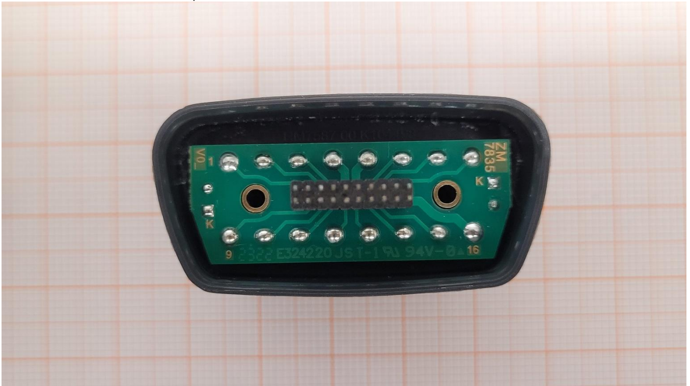
Photo No. 18: radiated test sample
