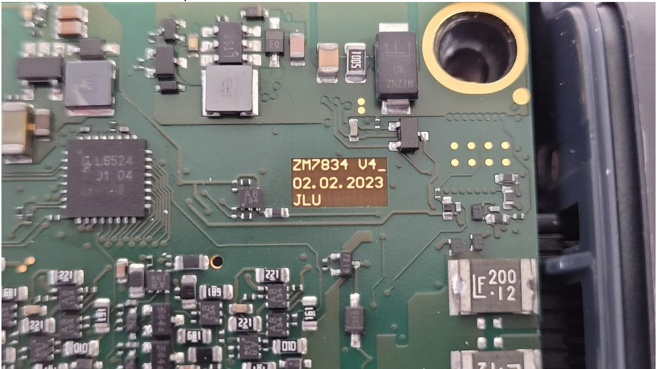
Photo No. 15: radiated test sample
