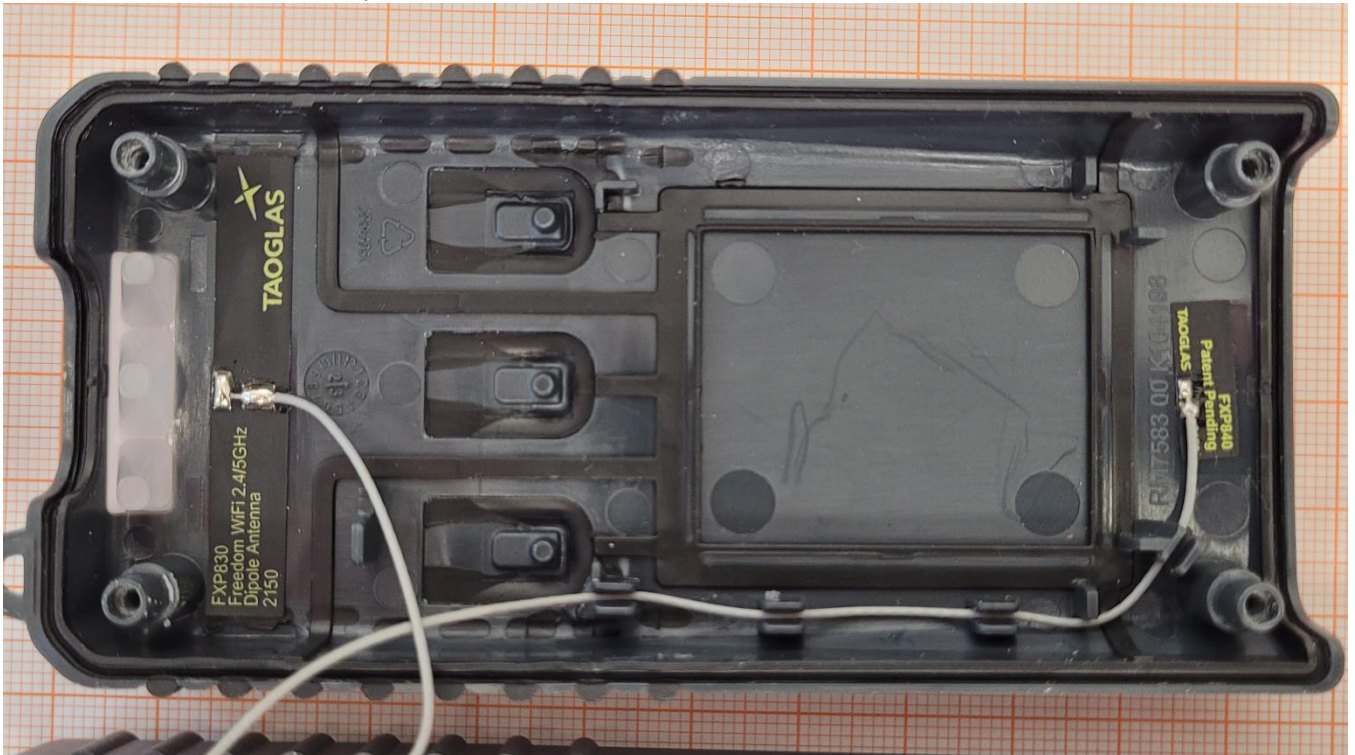
Photo No. 9: radiated test sample
