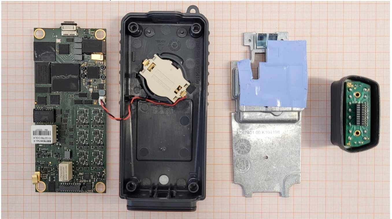
Photo No. 20: radiated test sample
