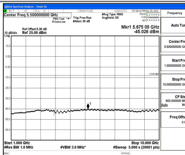
Band26-10MHz-16QAM-26740-1RB#0-Range4:1000~10000MHz
