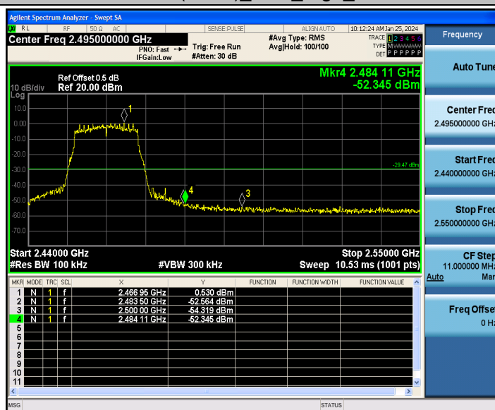
802.11n(HT20)_Ant2_High_2462
