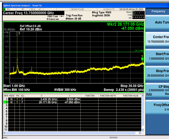
802.11n(HT20)_Ant2_2437_0~Reference
