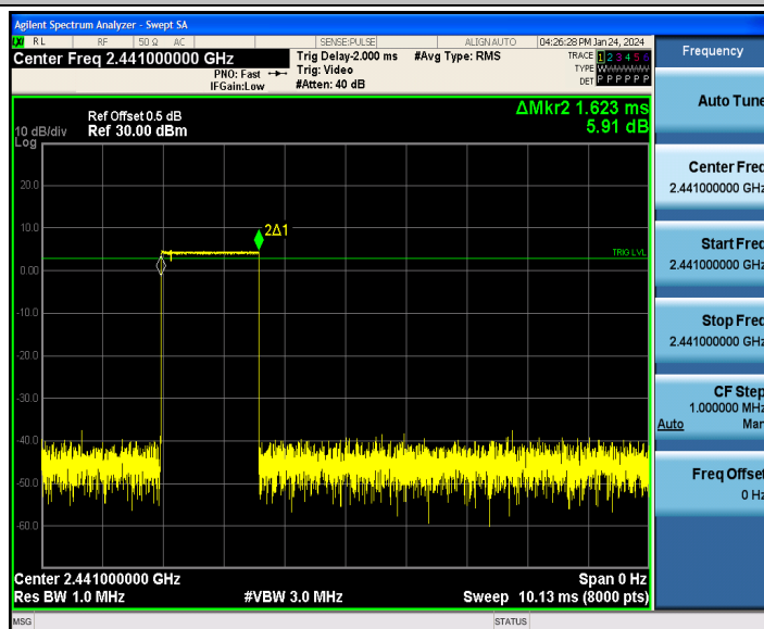
8-DPSK_8-DPSK_2441
