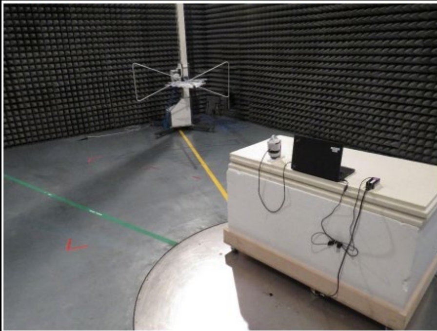
04 TEST SETUP - 30 MHz to 1000 GHz - EUT CONFIGURATION 2
