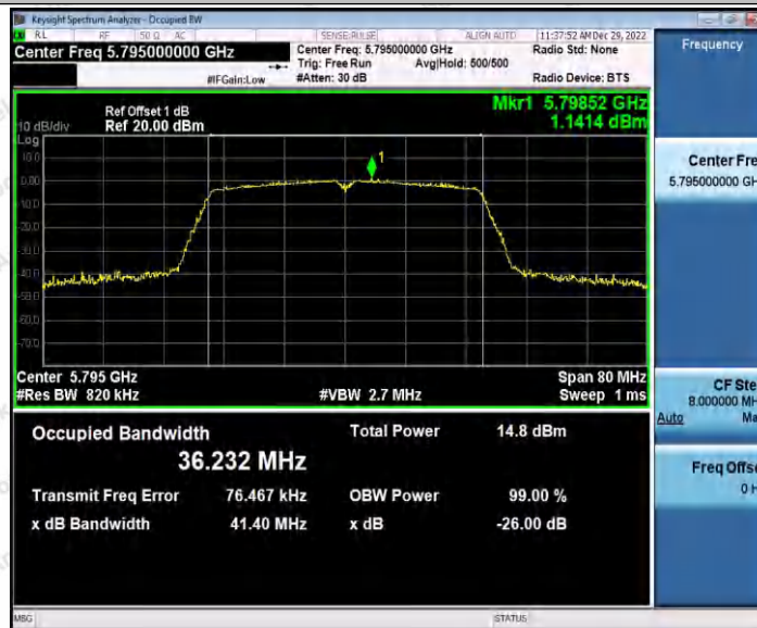
11AC40SISO_Ant3_5795
