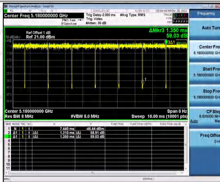
11A_Ant3_5180
