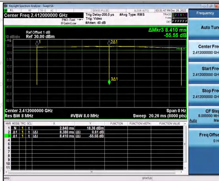
11B_Ant3_2412
