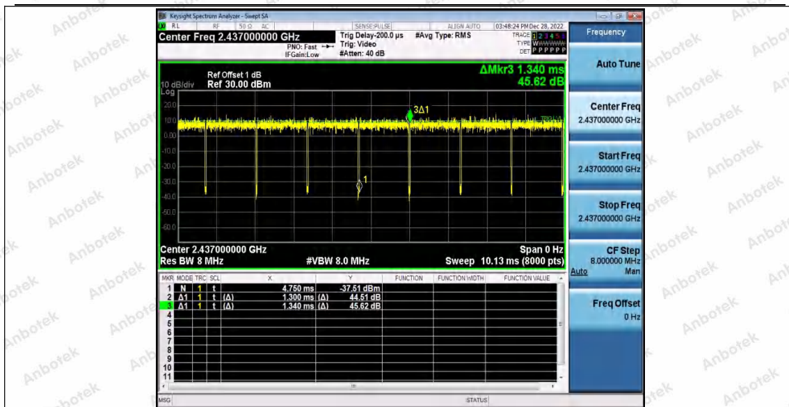
11N20_Ant3_2437
