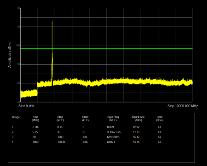
Band2 QAM16 BW=20MHz Channel=18900 RB Size=100 Position=#0
