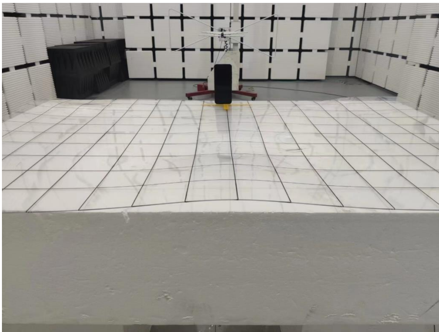
Radiated Spurious Emission Test Setup Photo - Below 1GHz
