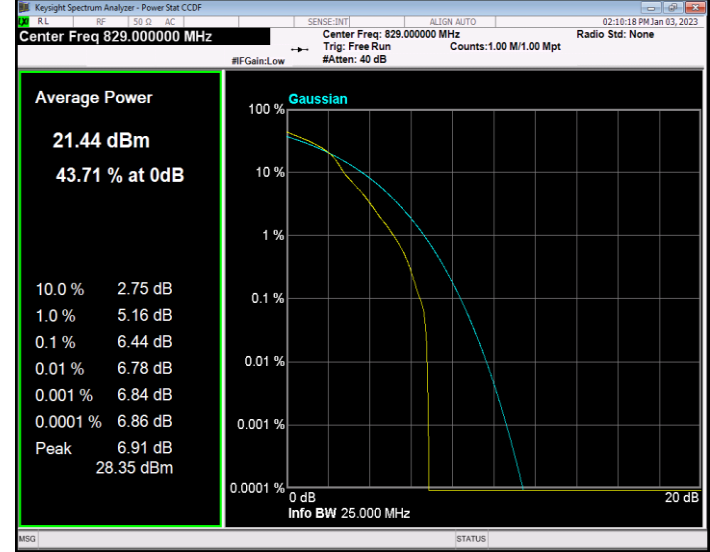
Band5 QAM16 BW=10MHz Channel=20525 RB Size=1 Position=#0
