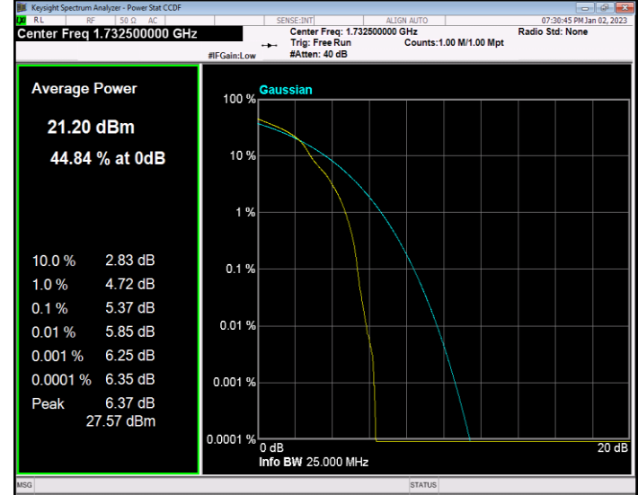
Band4 QAM16 BW=20MHz Channel=20300 RB Size=1 Position=#0
