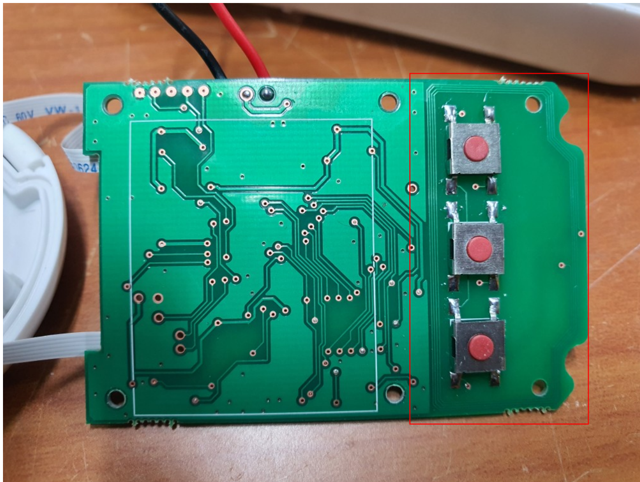
ANTENNA(RFID Pattern Ant 40 * 25 mm)
