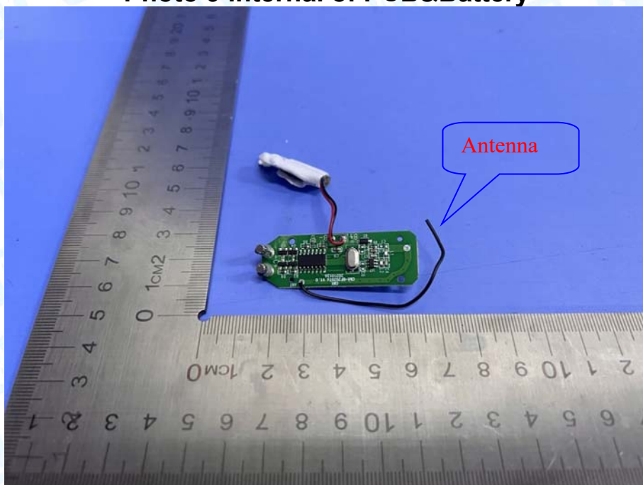
Photo 9 Internal of PCB&Battery
