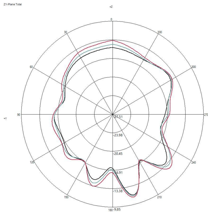
(2) Y-Z Plane (unit:dBi):
