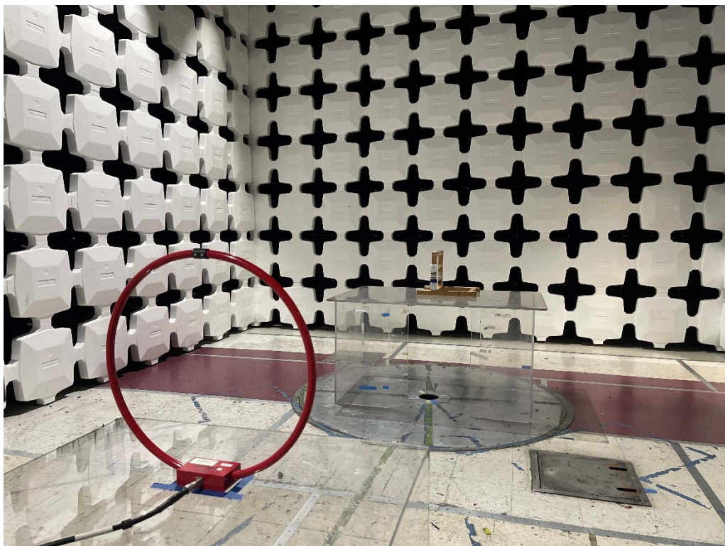
Radiated Emission Test below 30MHz Front View
