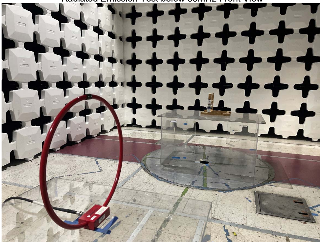
Radiated Emission Test below 30MHz Rear View
