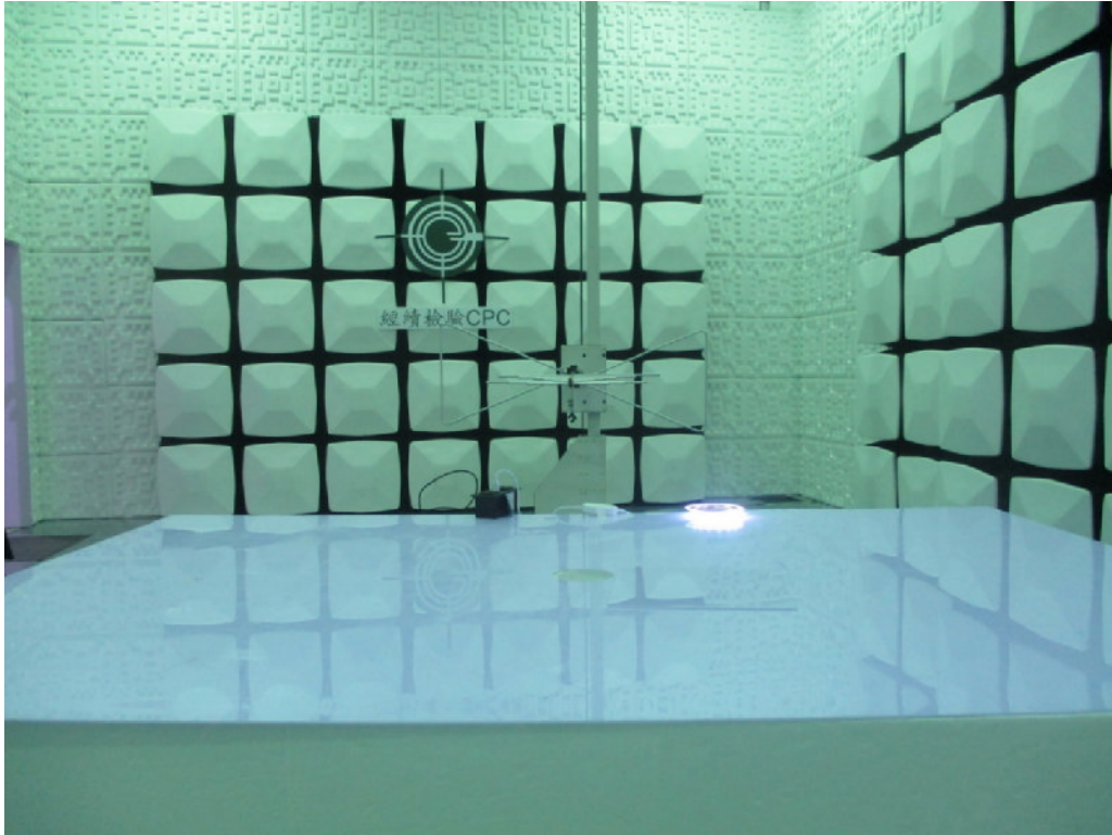
Setup Photo FCC ID: 2A9RHS4T01
