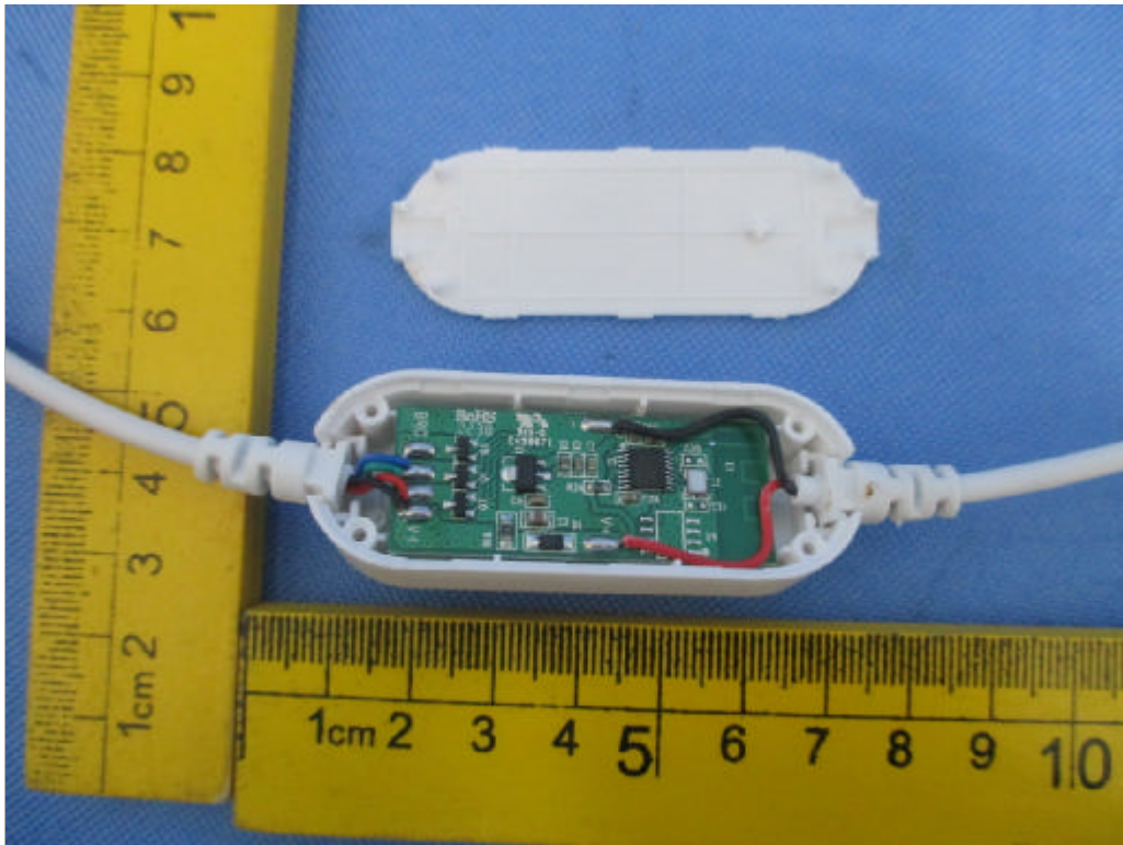
Internal Photo FCC ID: 2A9RHS4T01
